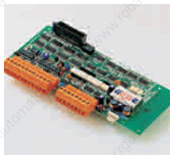
Analogue input board 4 inputs, 10bit resolution
