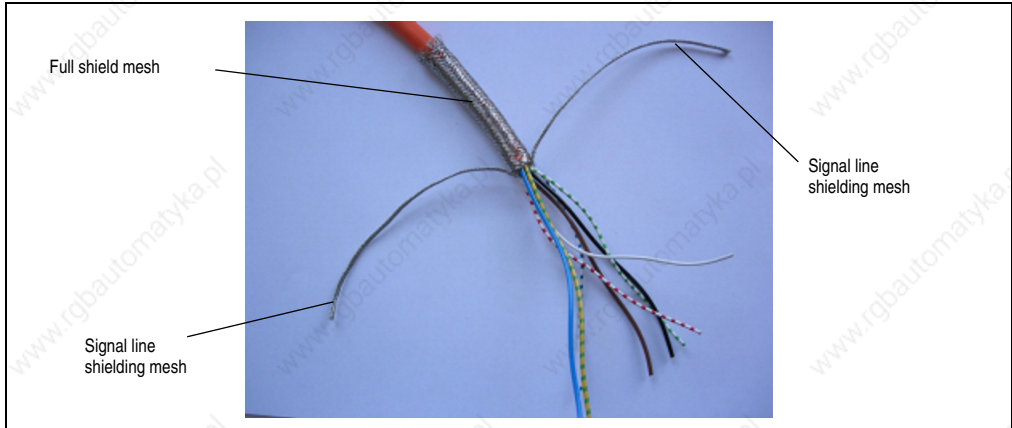
Figure 22: Cable end without stranding elements
