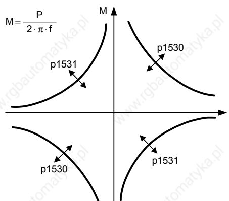
Power limitation (motoring, regenerative)
