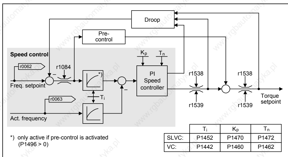
Fig. 3-105 Speed controller
