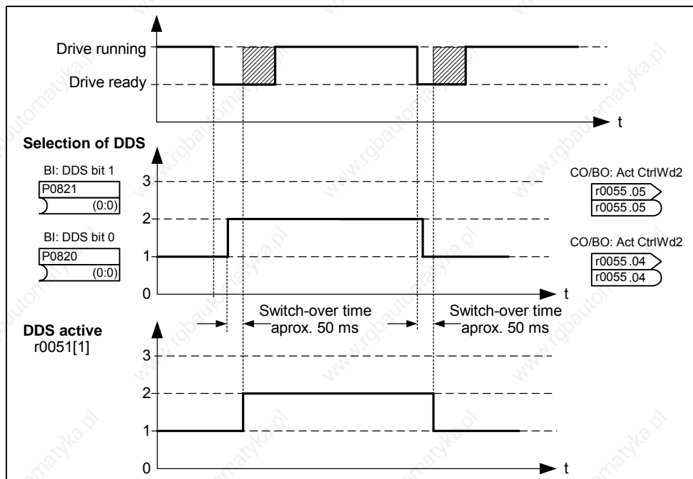
Fig. 3-12 Changing-over DDS
