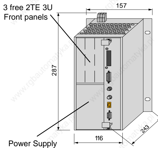
Figure 33 PAM Panel Mount Chassis
