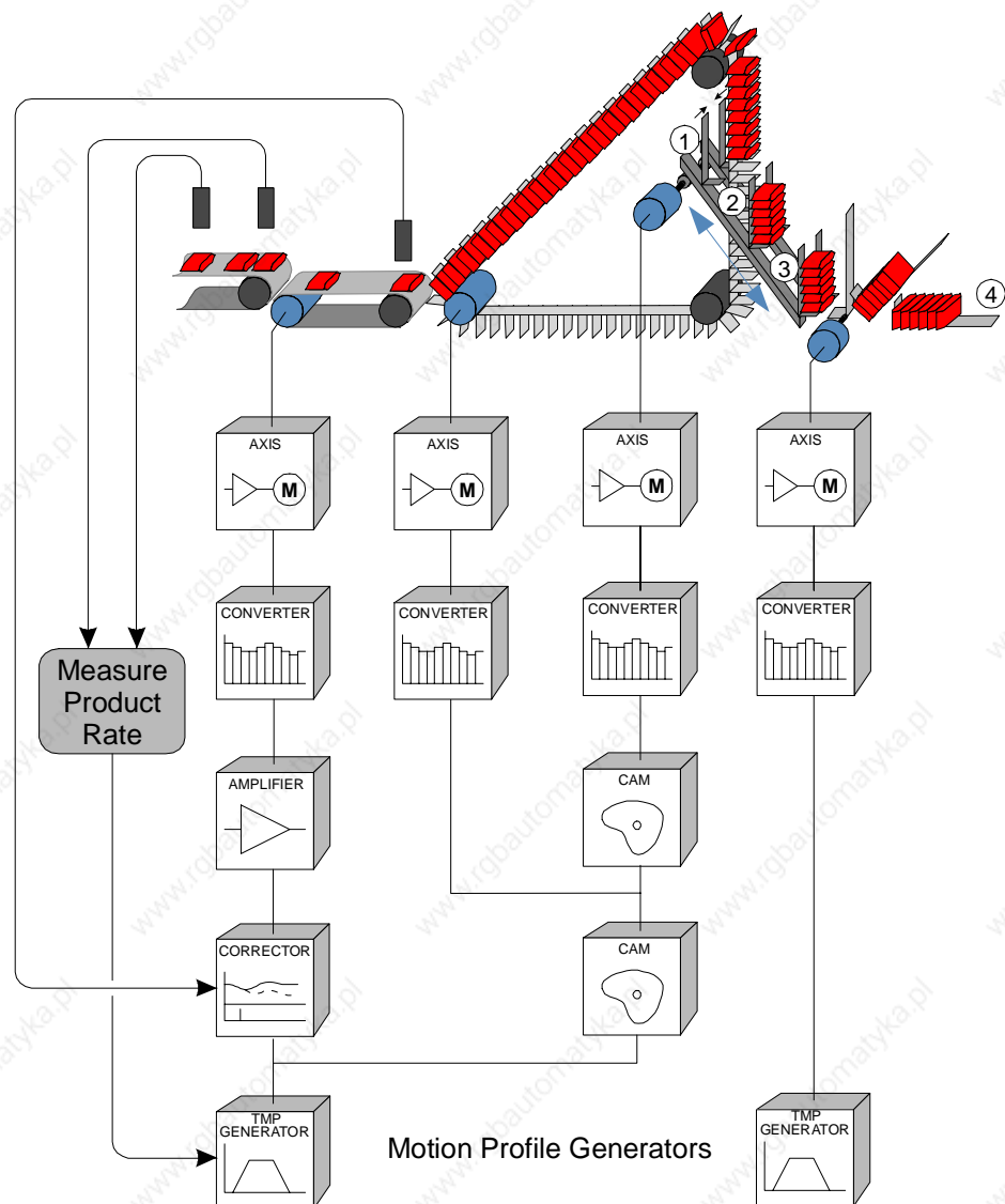
Figure 23 Packaging Machine Diagram
