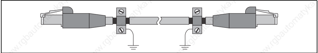
Figure 112: Grounding the POWERLINK cable shielding
