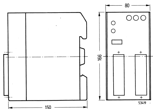
Fig. 23 383 Timer/counter module
