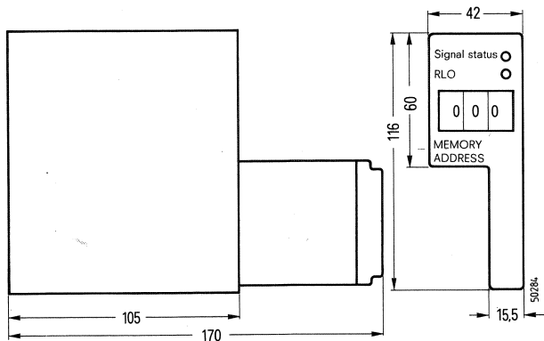
Fig. 21 332 Test adapter
