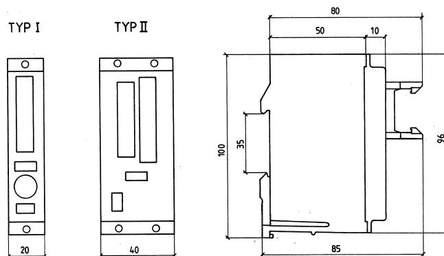
Fig. 24 Adapter blocks for 381 timer/counter module
