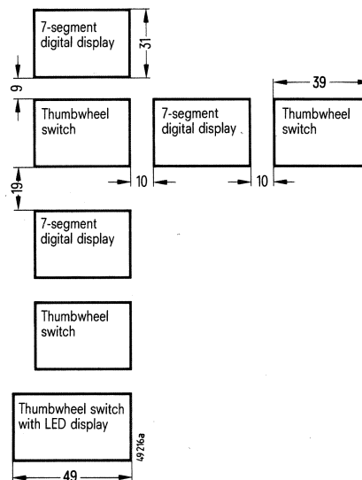
Fig. 27 Panel cutouts for thumbwheel switches with and without LED display and 7-segment digital display
