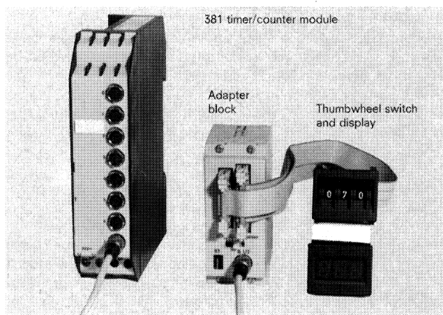
Fig. 7 381 Timer/counter module with components
