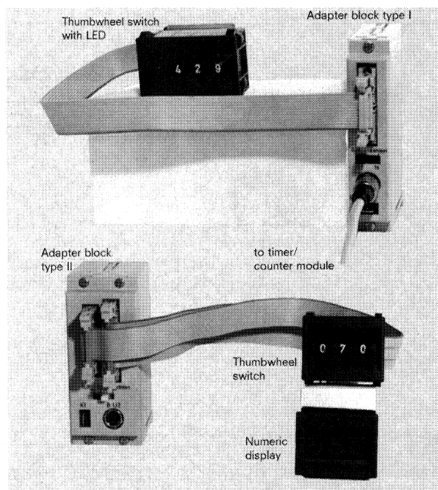
Fig. 8 382 Adapter blocks with accessories
