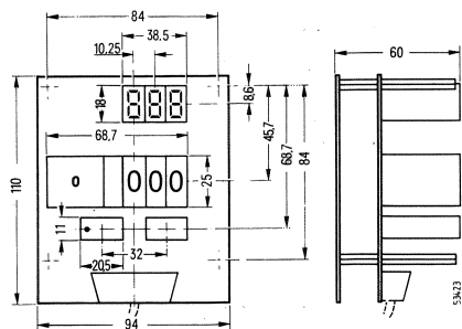
Fig. 25 Operator's panel for 383 timer/counter module
