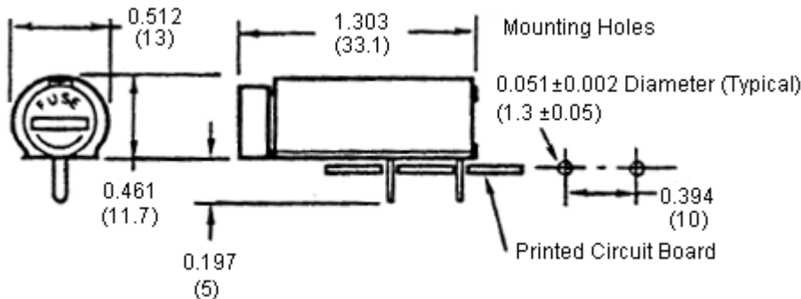
PCB Horizontal Mount Fuse holder
