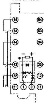
G7SA-4A2B Mounted
