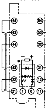
G7SA-3A3B Mounted
