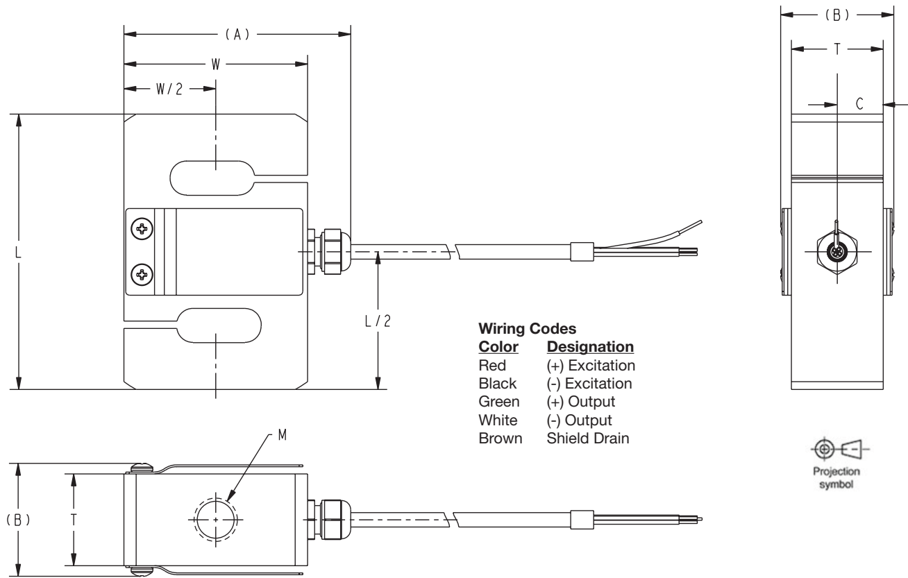
Figure 2. Model 151 & 152 Dimensions
