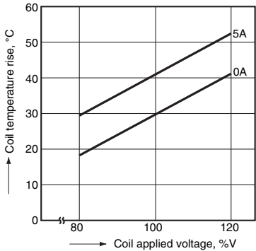
3.-(3) Coil temperature rise (2 Form A) Tested sample: DSP2a-DC12V, 5 pcs.
