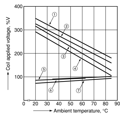
4.-(1) Ambient temperature characteristics (1 Form A type)
