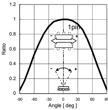
Fig.4 Directional Characteristics 1
