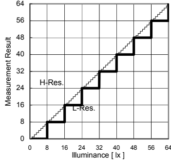
Fig.2 Illuminance - Measurement Result 1
