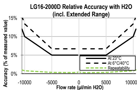
Figure 1: Flow meter accuracy and repeatability across the flow range. Relative error in % of measured value (left column) and absolute error in \mu\text{l/min} (right column) for H 2 O.
