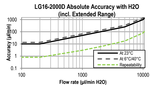
Figure 1: Flow meter accuracy and repeatability across the flow range. Relative error in % of measured value (left column) and absolute error in \mu\text{l/min} (right column) for H 2 O.
