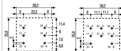
62.22 - 0300 Copper side view 62.23 - 0300 Copper side view
