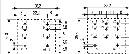
62.22 Copper side view 62.23 Copper side view
