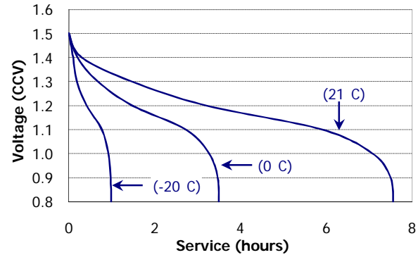
Constant Current Performance 250 mA Discharge (-20°C / 0°C / 21°C)
