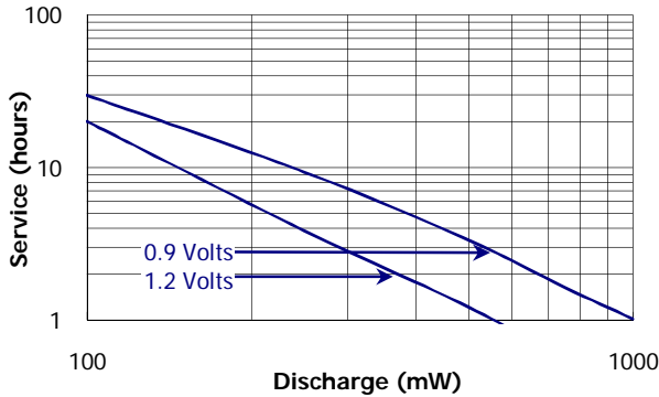
Constant Power Performance Typical Characteristics (21°C)
