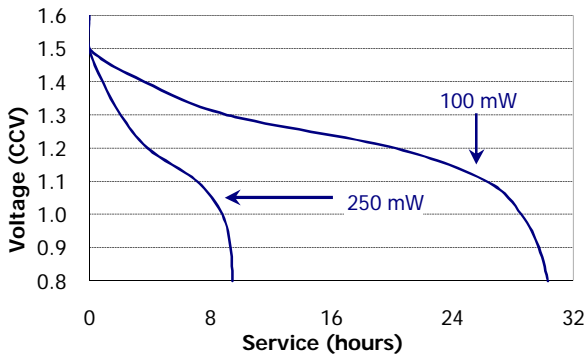
Constant Power Performance Discharge Characteristics (21°C)
