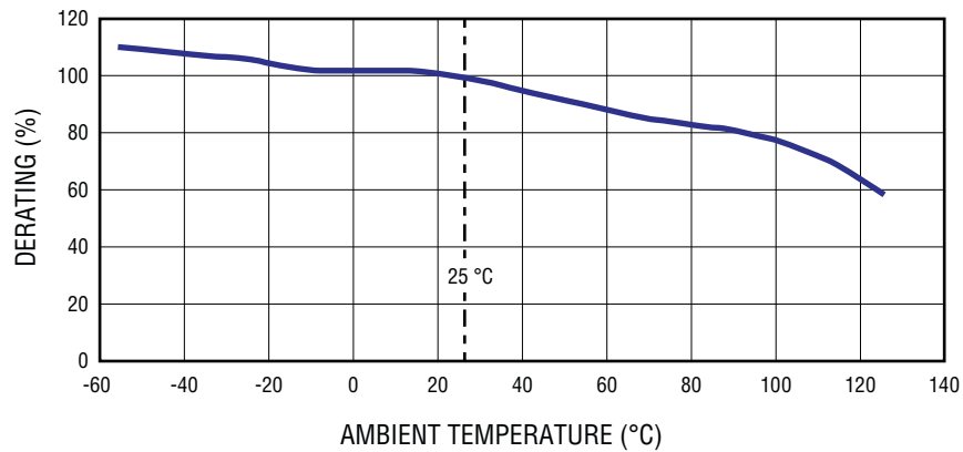
Current Rating Thermal Derating Curve
