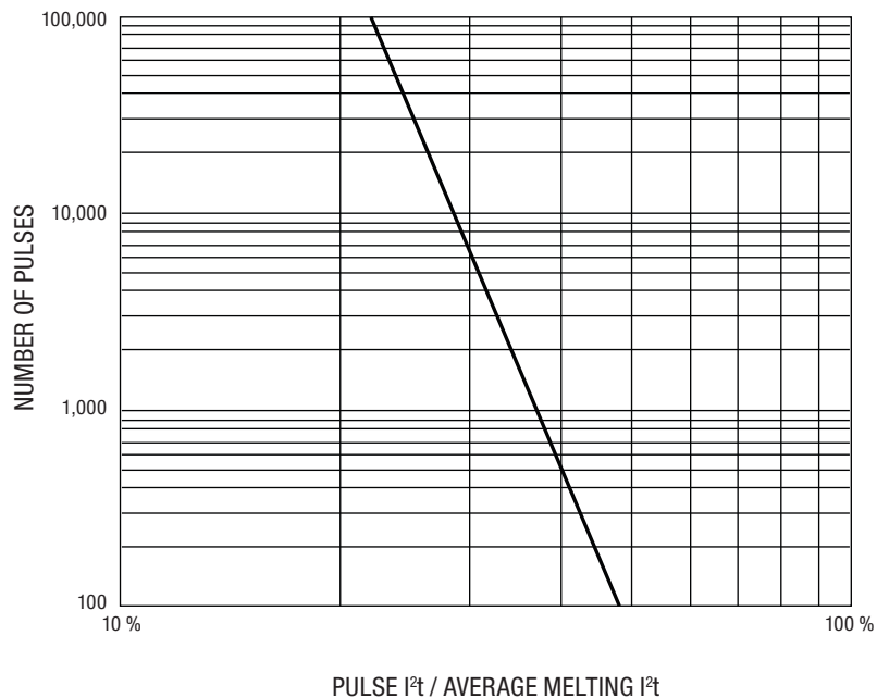
Pulse Cycle Withstand Capability
