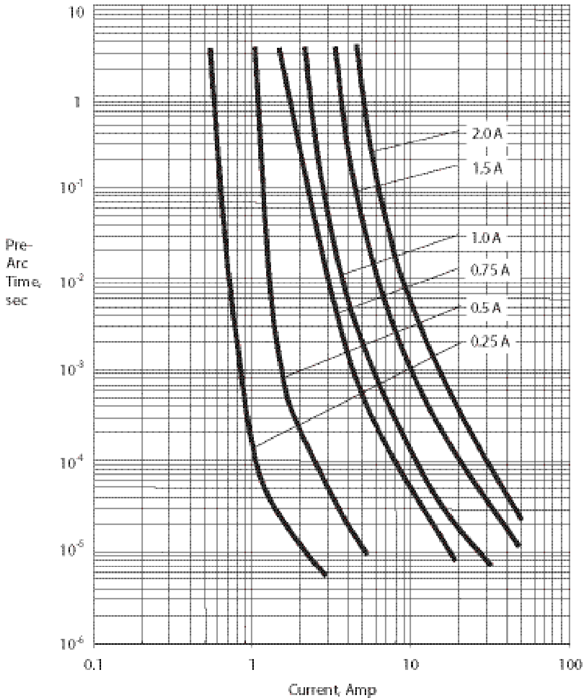
Fuse Time – Current Characteristics for Type MCF0402E (Typical)
