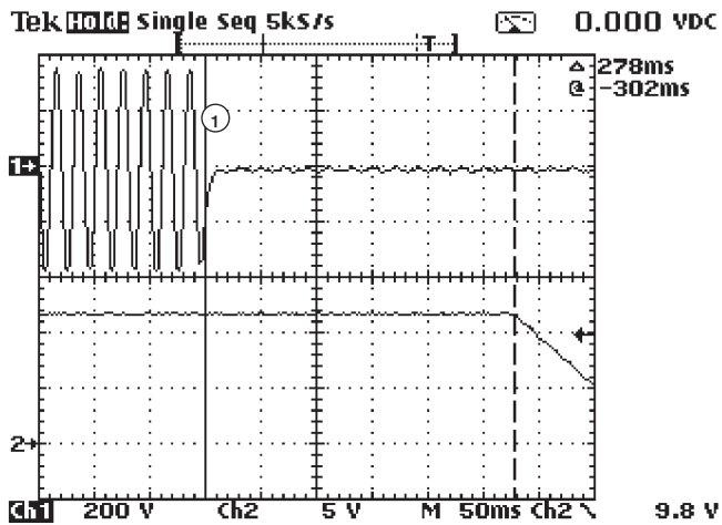
Figure 5 V2 278 ms (Full load at 90 VAC input)
