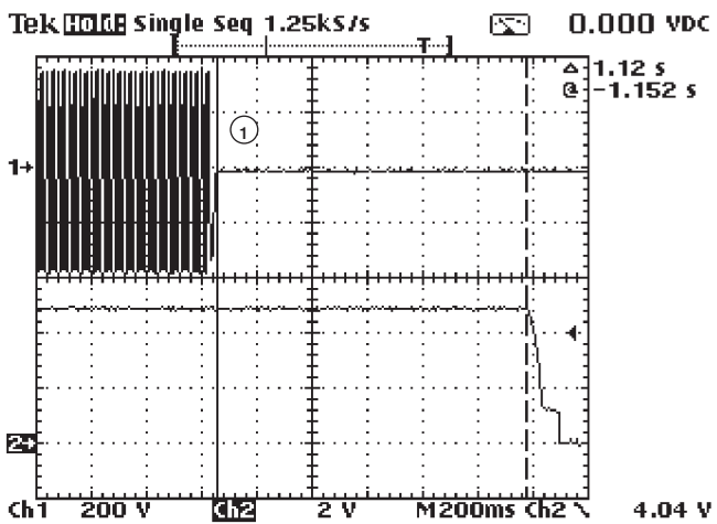
Figure 6 V3 1.12 s (Full load at 90 VAC input)
