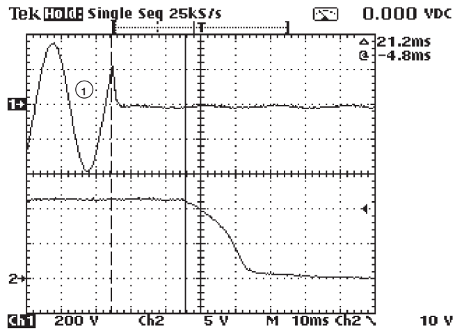
Figure 4 V1 21.2 ms (Full load at 90 VAC input)
