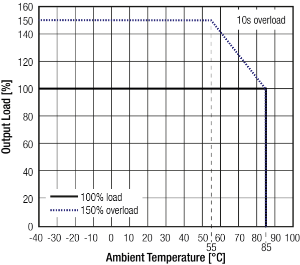
Derating Graph
