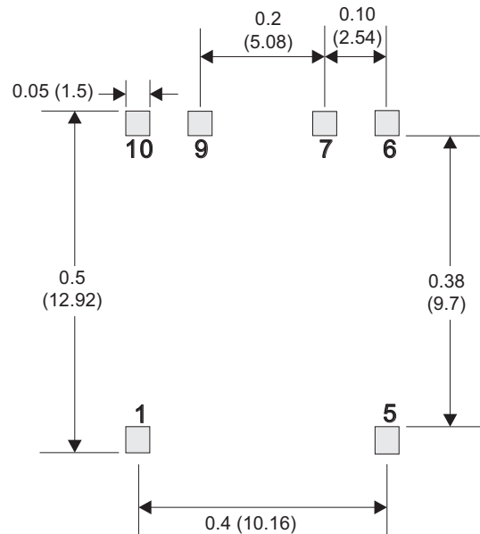
Solder Pad Dimension
