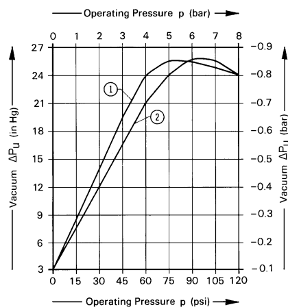
Vacuum as a function of operating pressure
