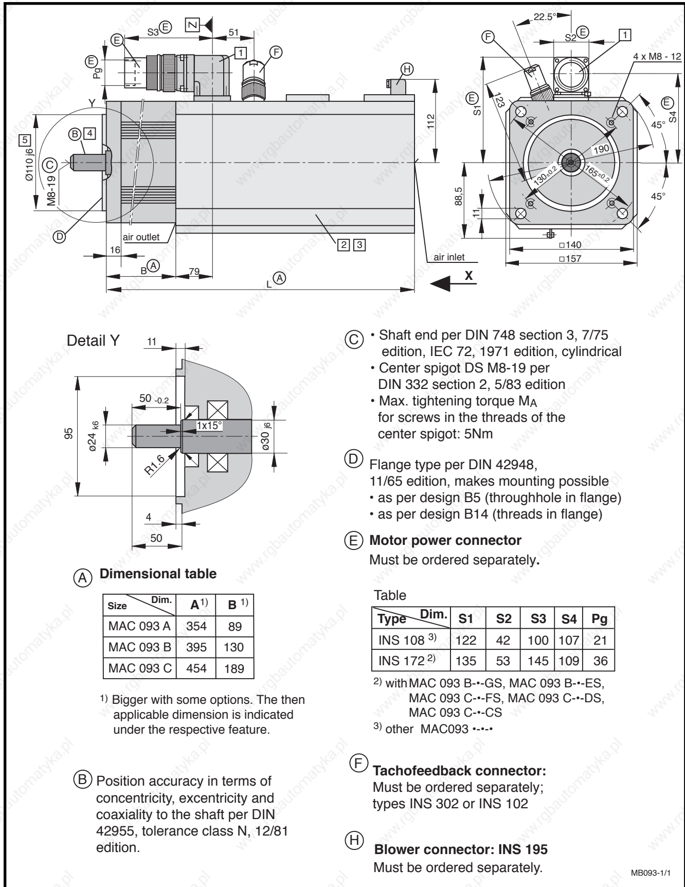
Fig 6.19: Dimensional data - MAC 093 (axial cooling)
