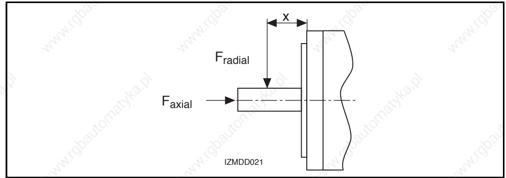
Fig 3.8: Shaft load
