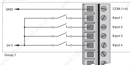
Sink Circuit:
