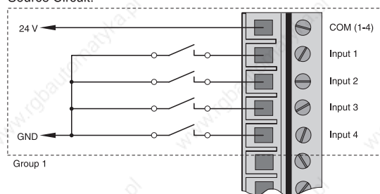
Source Circuit:
