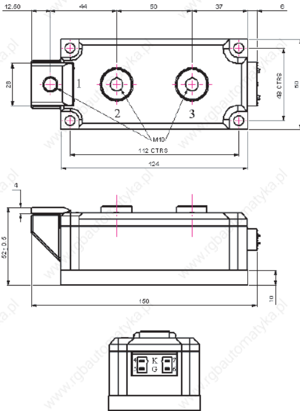
X200 Metal-can
