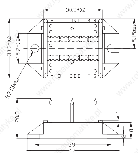
X101 ECO-PAC1
