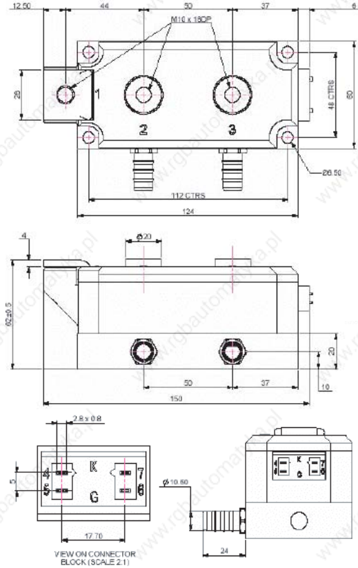
X202 BOD-Package
