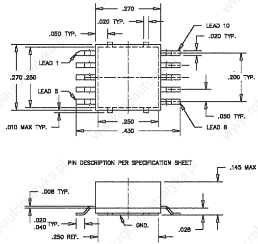
Package 84
