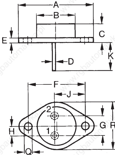
X203 TO-204 AE
