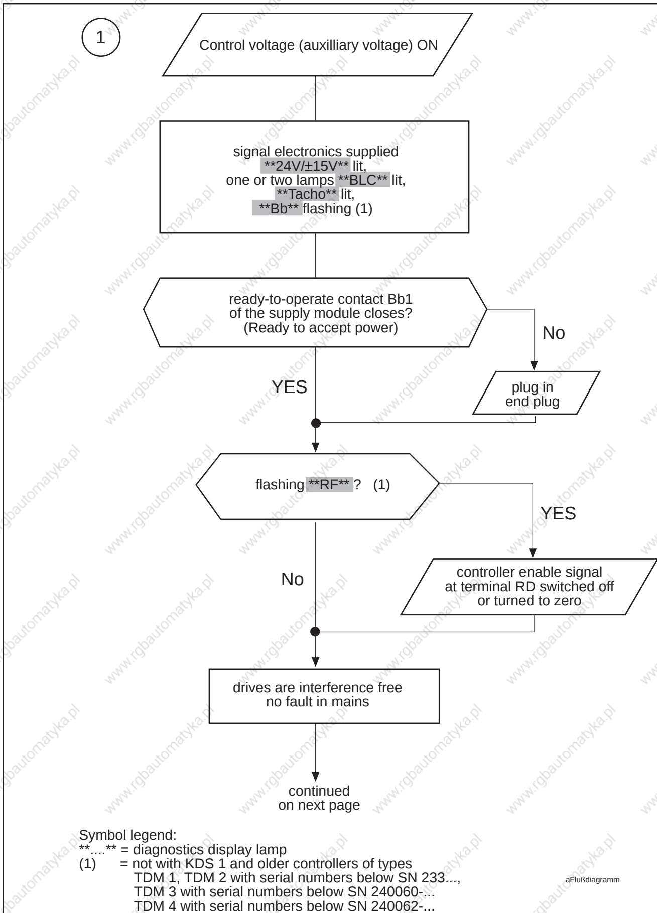
Figure 72: Power-Up Sequence
