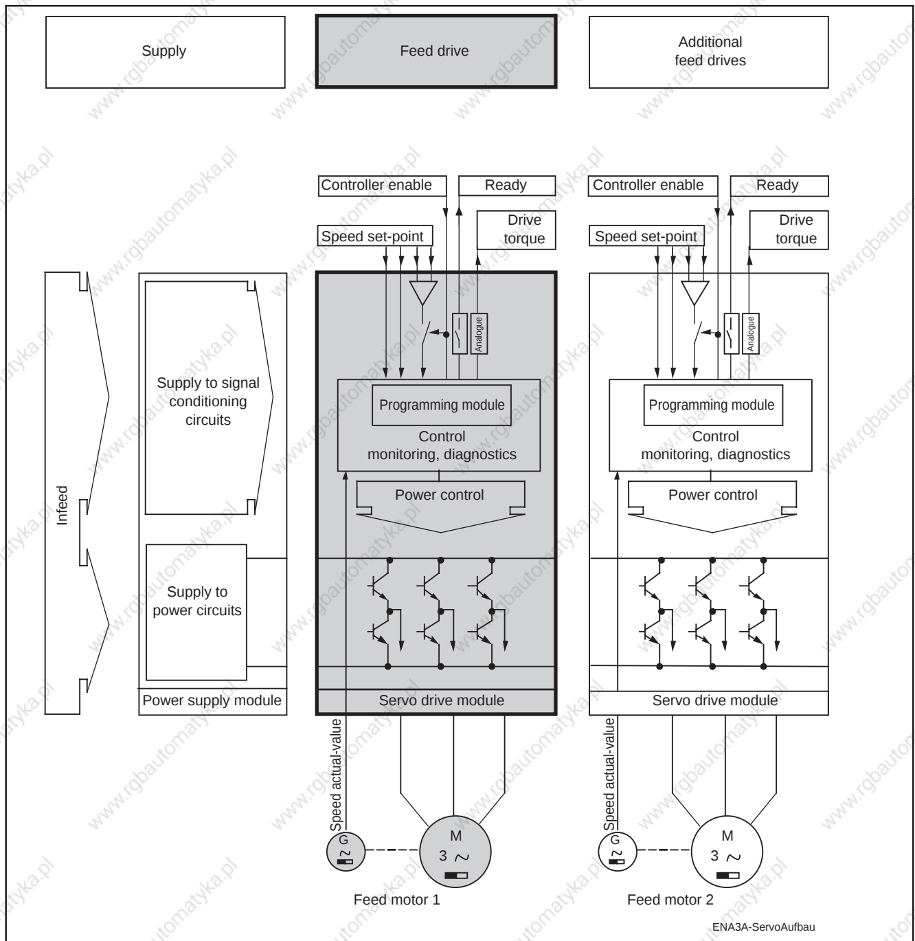
Fig. 2: modular construction
