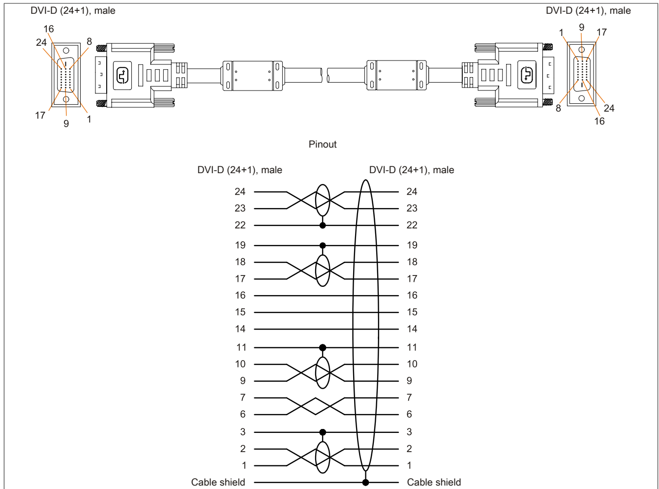
Figure 102: 5CADVI.0xxx-00 - Pinout
