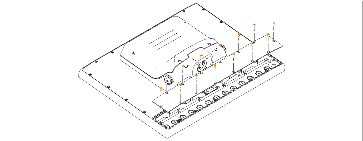
Figure 78: Removing the back cover
