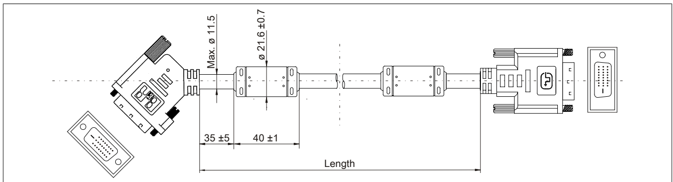
Figure 107: 5CASDL.0xxx-01 - Dimensions
