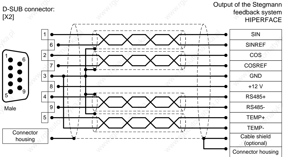
Figure 18: Pin configuration [X2]: In case of the Stegmann (HIPERFACE) encoder evaluation module
