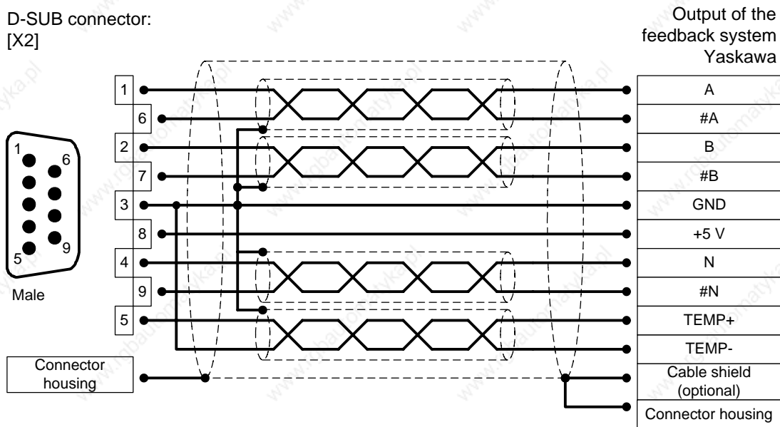
Figure 19: Pin configuration [X2]: In case of the Yaskawa (SGM, Sigma 1) Incremental encoder evaluation module
