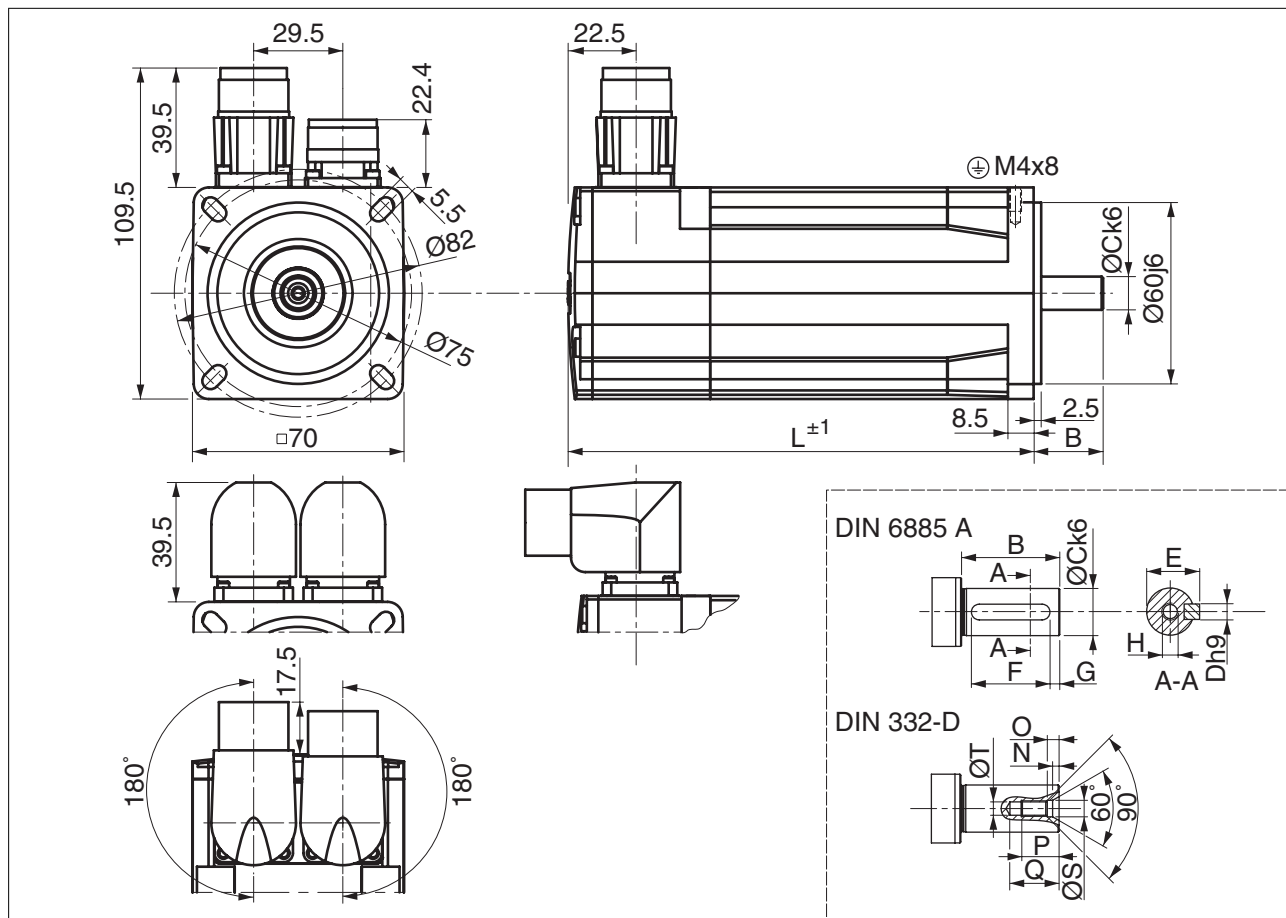
Figure 2: Dimensions BMH070
