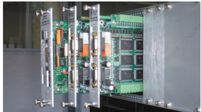
12 AXIS (SLM) WITH UMAC
