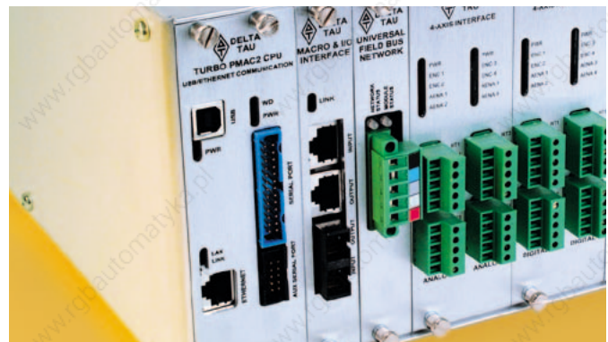
TURBO UMAC WITH USB AND ETHERNET
