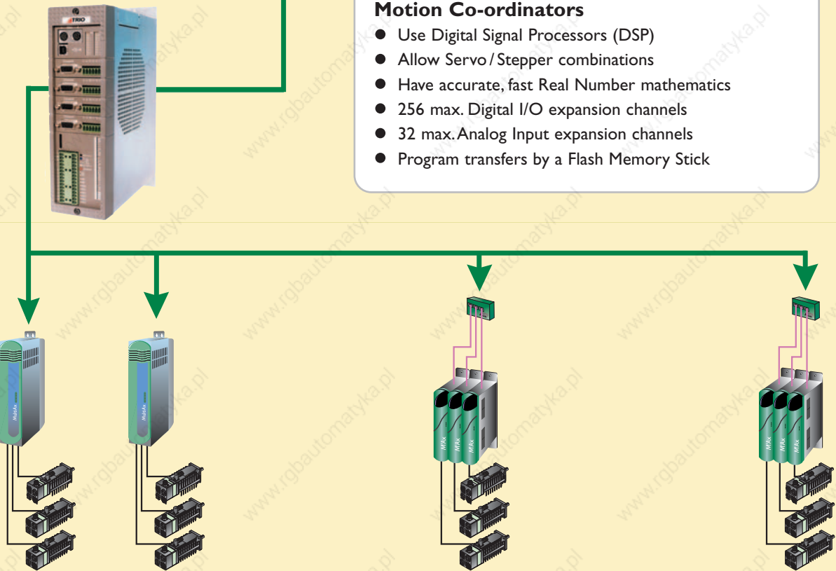
Up to 12 Digital Drives can be controlled with (SLM) Daughter Boards in MC224 Motion Coordinator
