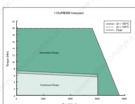
115UMB300 Unimotor
