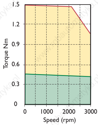
DCM 6C 30/14 Maestro DCD 140* 8/16
