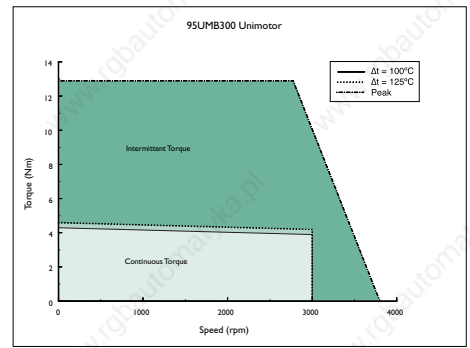
95UMB300 Unimotor
