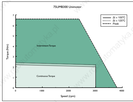
75UMB300 Unimotor
