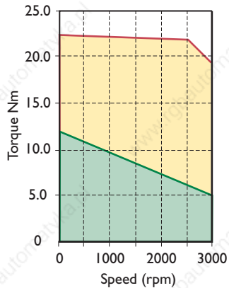
DCM 9B 30/20 Maxi Maestro 200* 25/50
