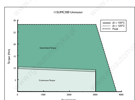
115UMC300 Unimotor
