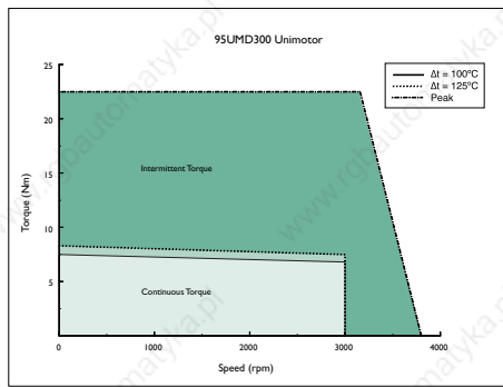
95UMD300 Unimotor
