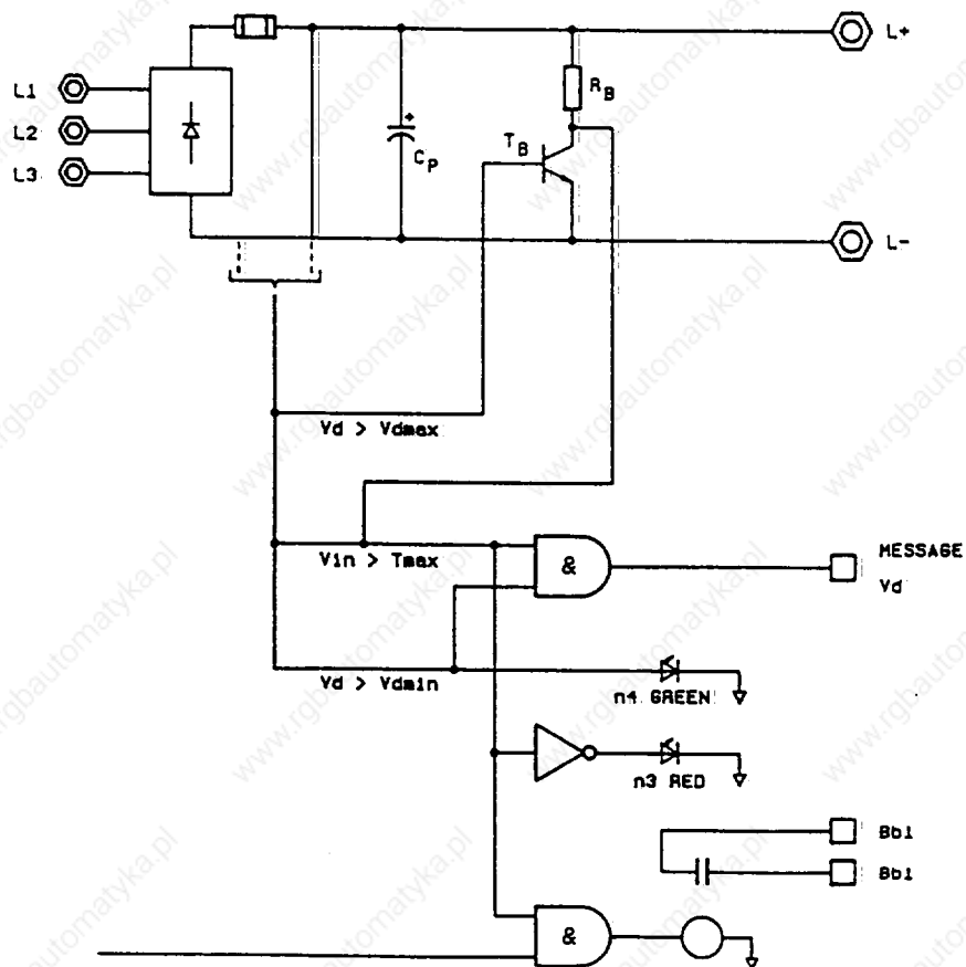
Figure 1-2. TVM Power Supply Schematic
