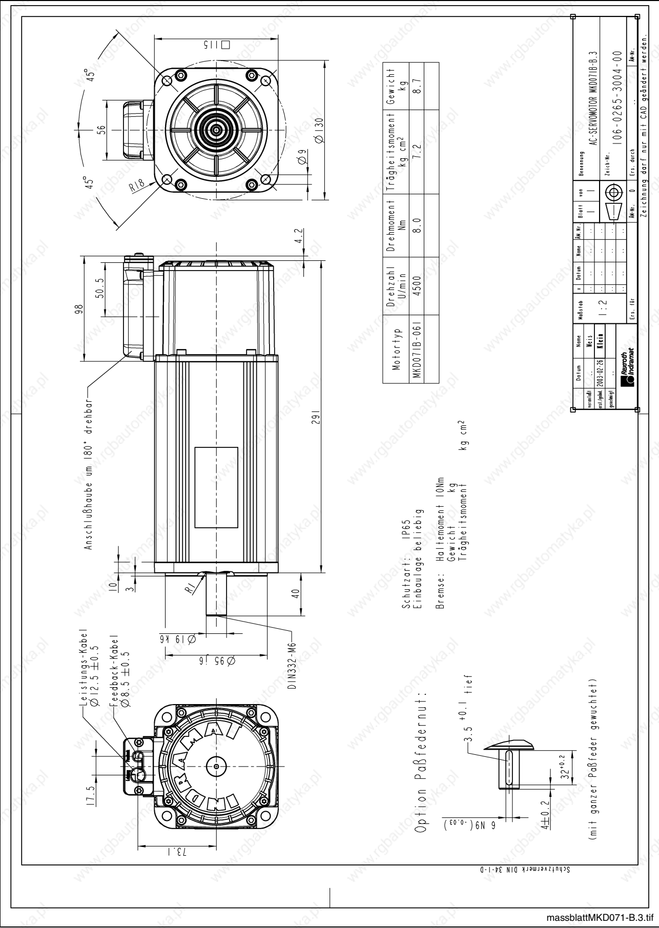
Fig. 8-10: Dimensional data MKD071 (holding brake 3)
