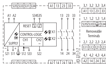
ESR4-NO-31...(AC 115/230 V)
