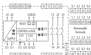
ESR4-NO-31...(AC/DC 24 V)
