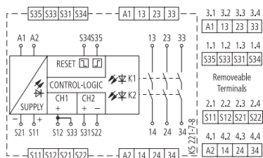
ESR4-NO-30...(AC/DC 24 V)
