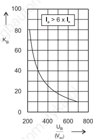
Reduction factor for total I 2 t-value
