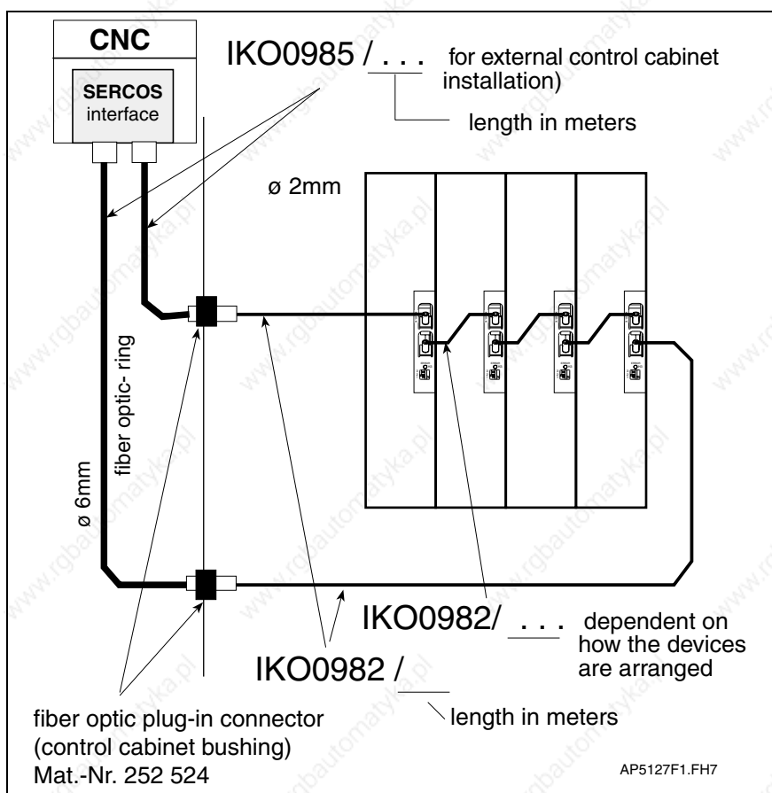
Fig. 4-180: Selecting standard fiber optic cables
