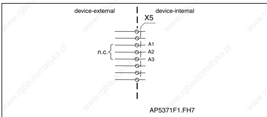
Fig. 6-40: Motor connection
