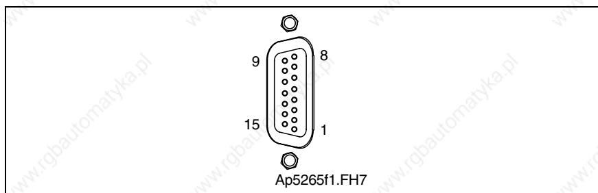
Fig. 5-44: Connector X4
