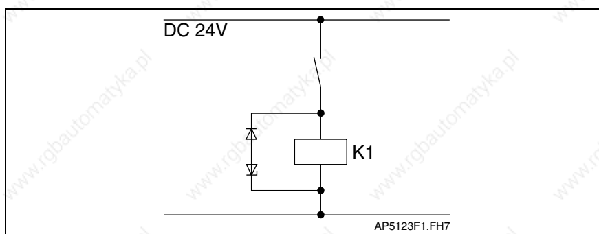
Fig. 11-1: Recommended protective circuits
