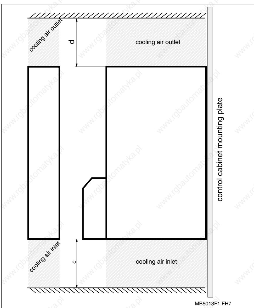
Fig. 12-10: Exit and entrance of cooling air
