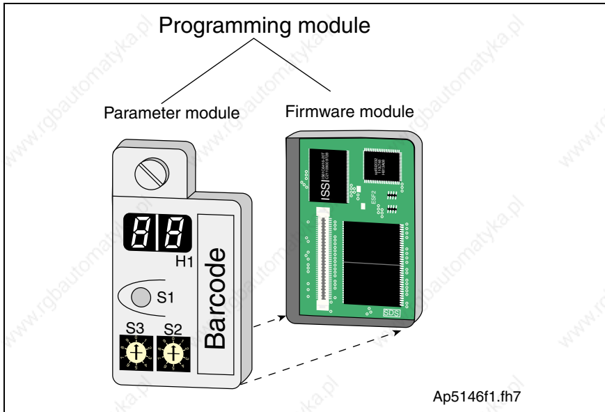
Fig. 15-5: Programming module
