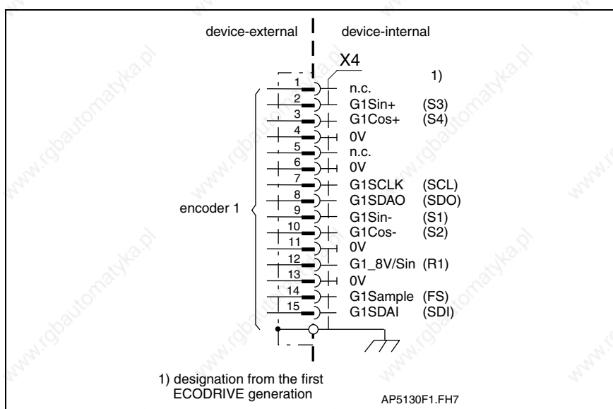
Fig. 5-47: Encoder 1
