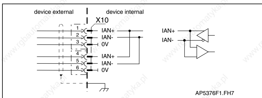
Fig. 4-136: Expansion interface
