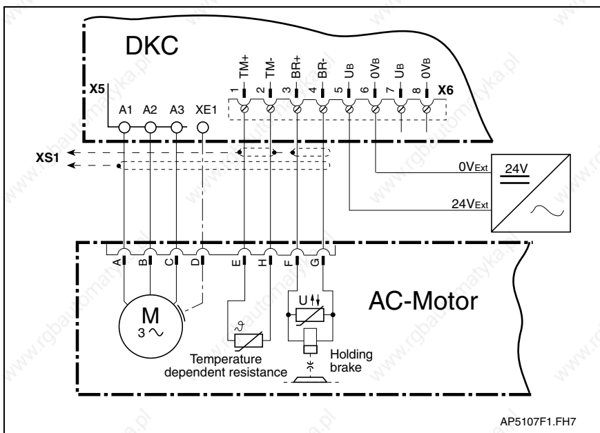
Fig. 4-106: Connection of motor cable, holding brake and temperature monitor for motors with connectors
