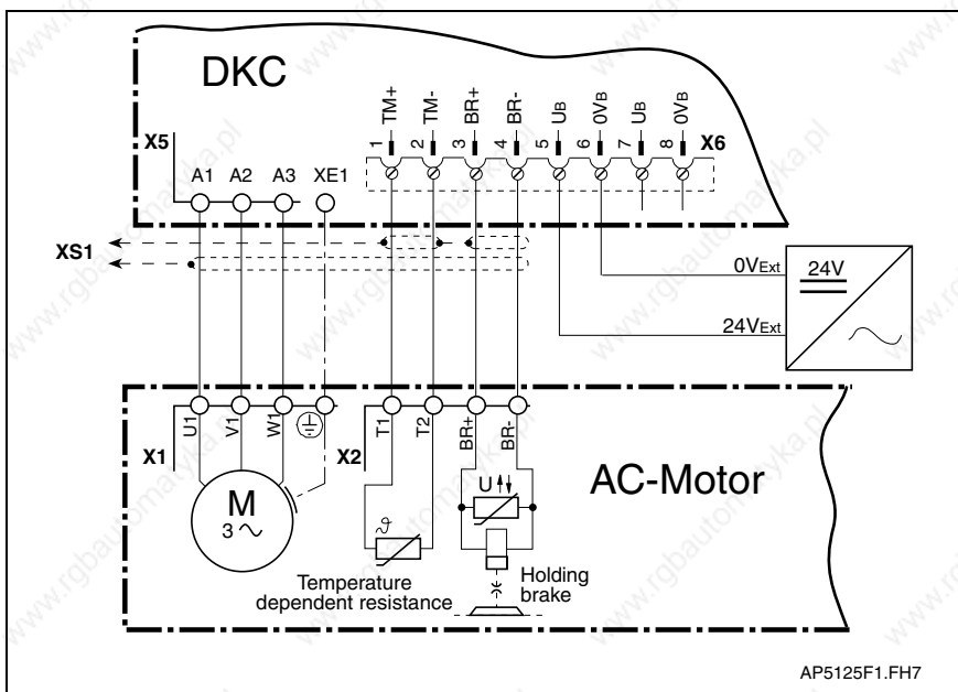
Fig. 4-107: Connection of motor cable, holding brake and temperature monitor for motors with connector box
