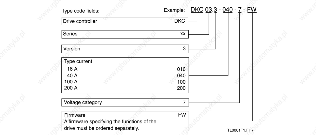
Fig. 1-5: Type code
