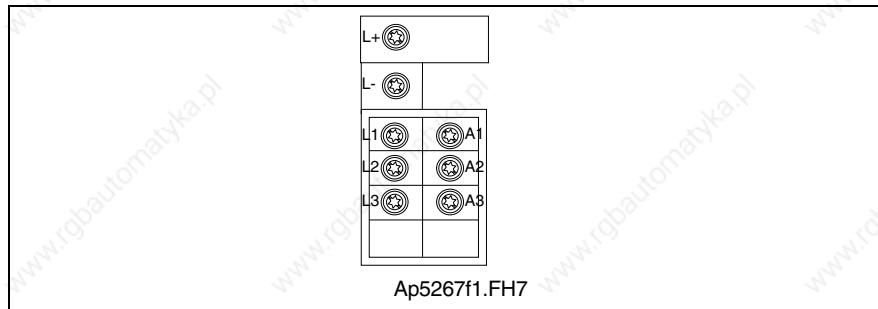
Fig. 7-8: Connector X5
