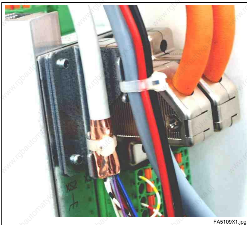
Fig. 16-25: Detail view X4, X8, XS2
