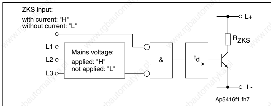
Fig. 6-25: Block diagram interlock ZKS/Mains
