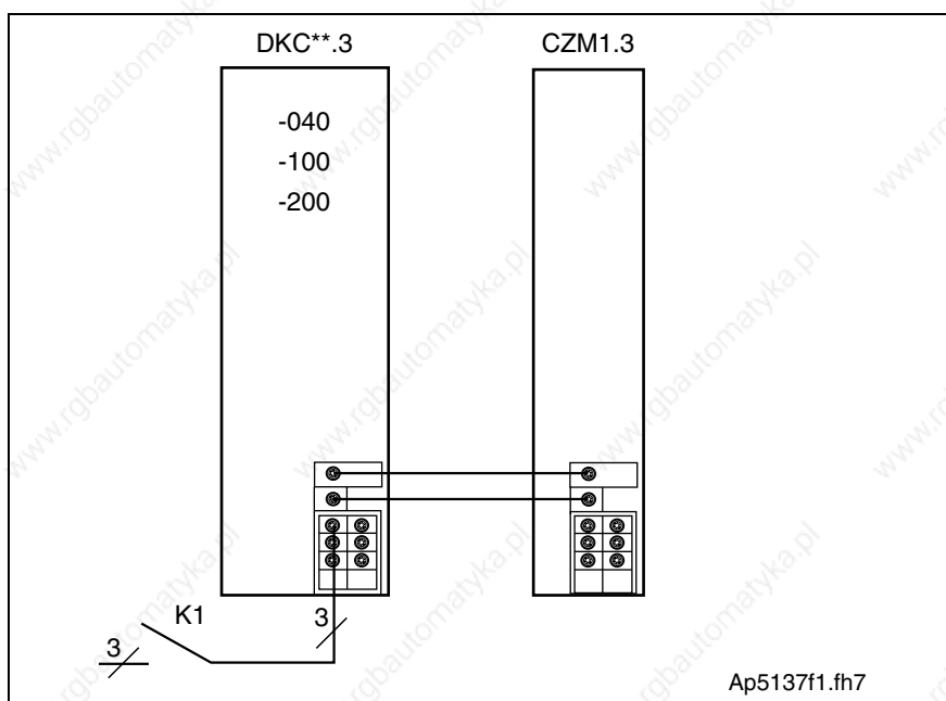
Fig. 7-13: Connection of auxiliary capacitance module CZM01.3
