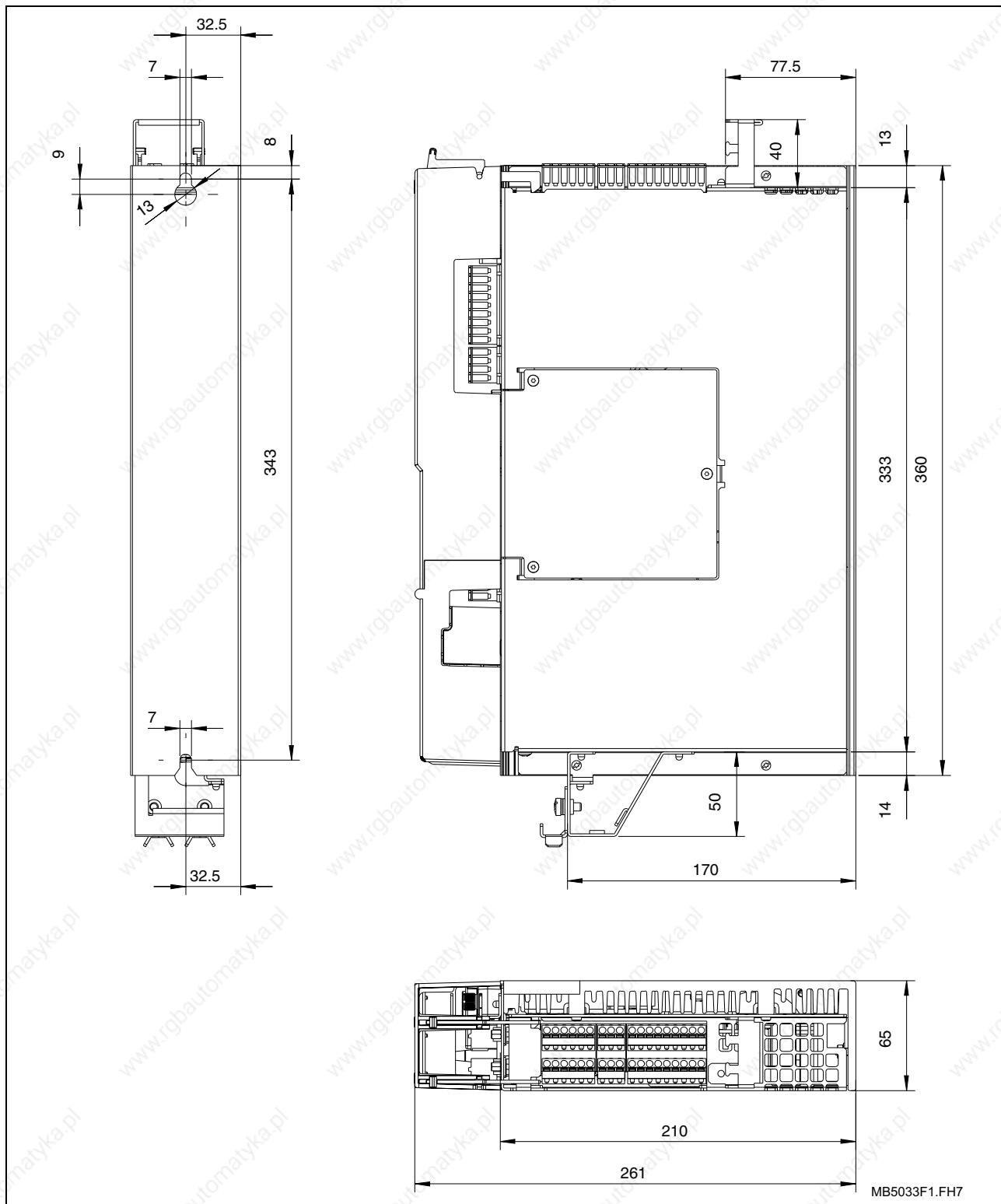
Fig. 4-1: Drive Controller DKC**.3-040-7-FW
