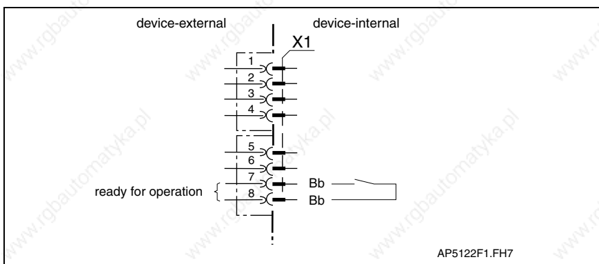
Fig. 6-16: Connections for ready to operate contact
