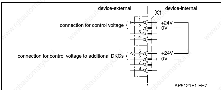
Fig. 4-51: Connections for control voltage
