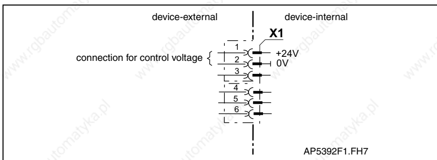
Fig. 5-25: Connections for control voltage
