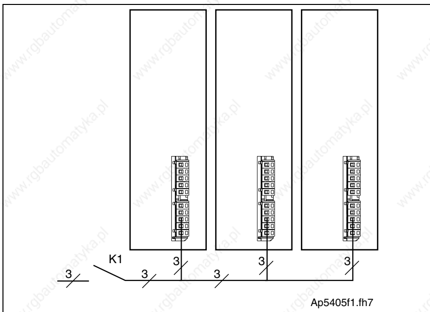
Fig. 5-11: Group supply
