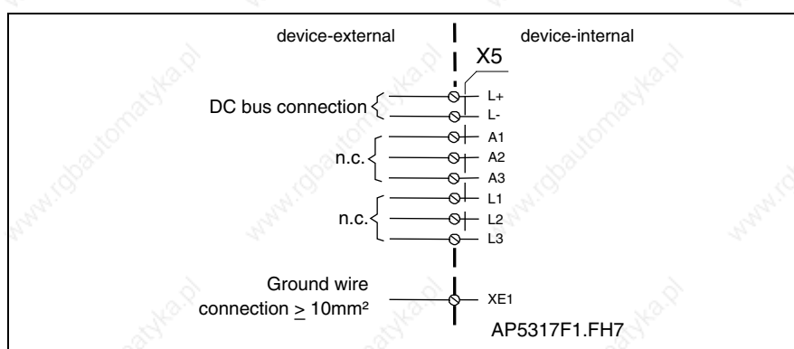
Fig. 7-12: DC bus connection of auxiliary capacitance module CZM01.3 – X5
