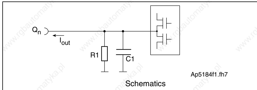
Fig. 4-217: Output circuit
