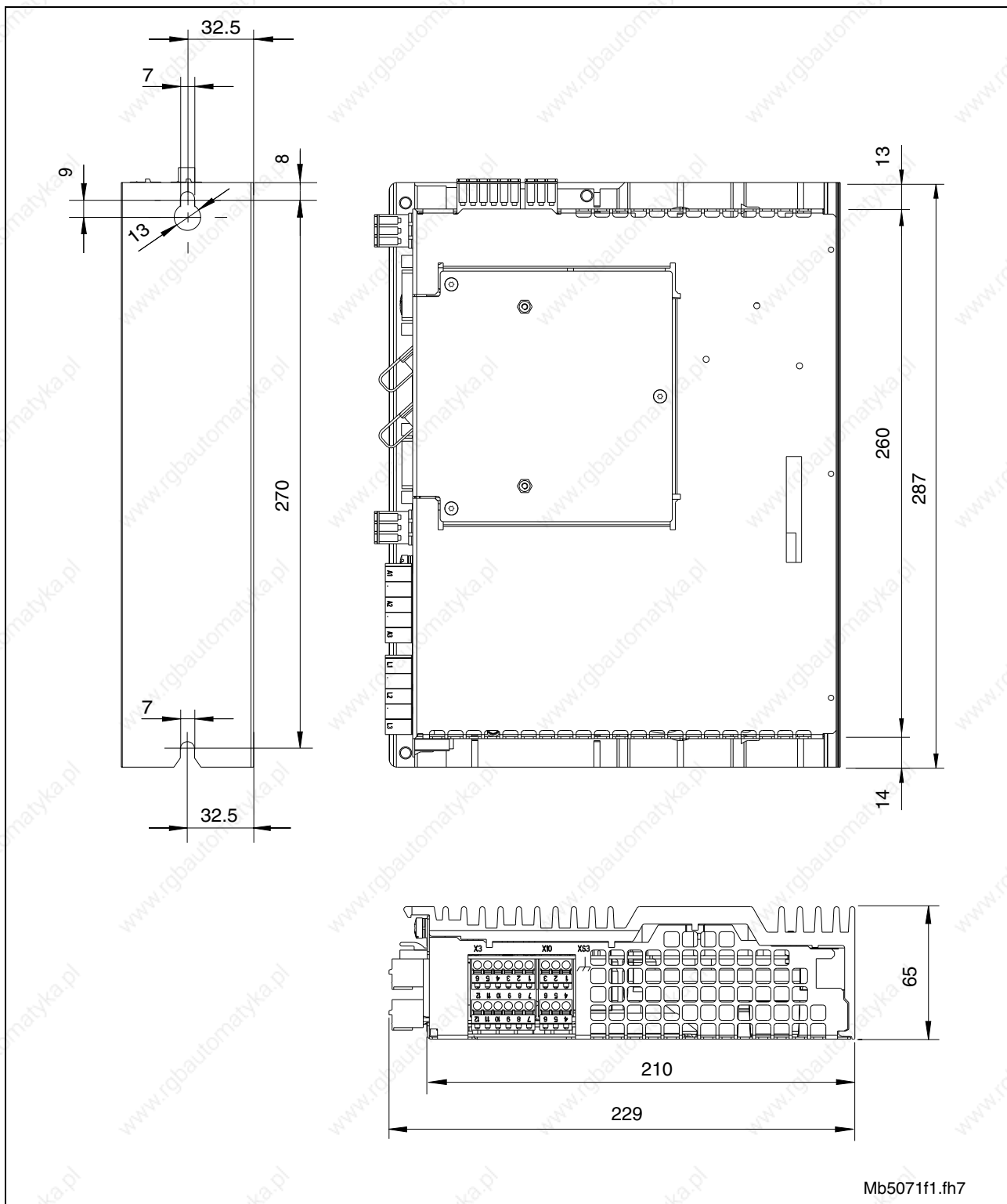
Fig. 5-1: Drive Controller DKC**.3-016-7-FW
