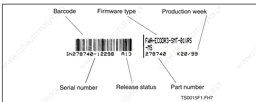
Fig. 14-4: Type plate
