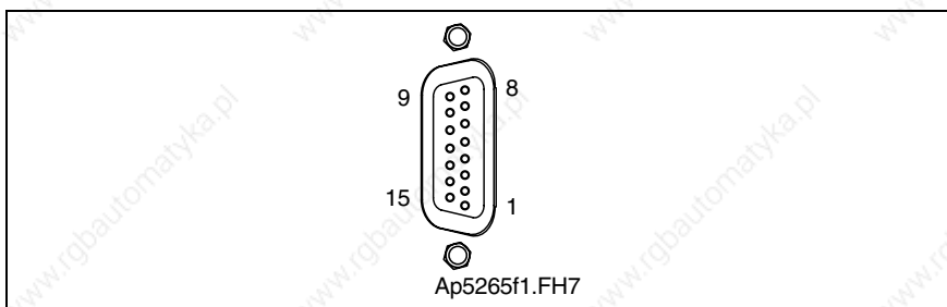
Fig. 4-81: Connector X4
