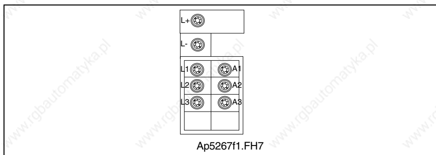
Fig. 4-89: Connector X5
