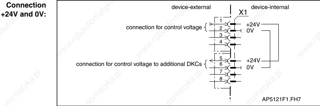
Fig. 6-14: Connections for control voltage
