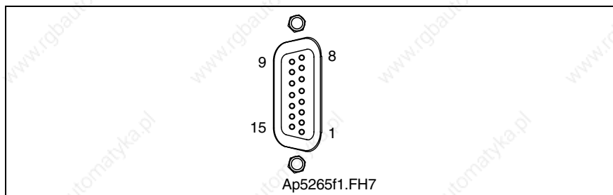
Fig. 5-30: Connector X2
