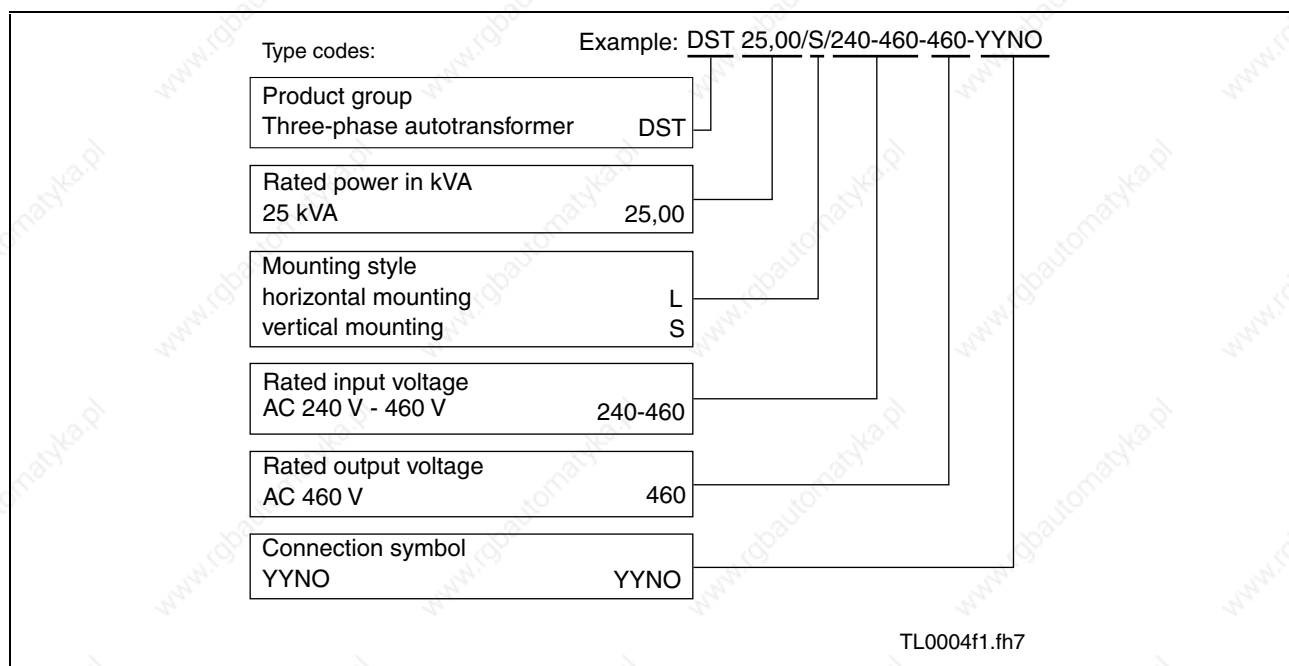
Fig. 10-3: Type code
