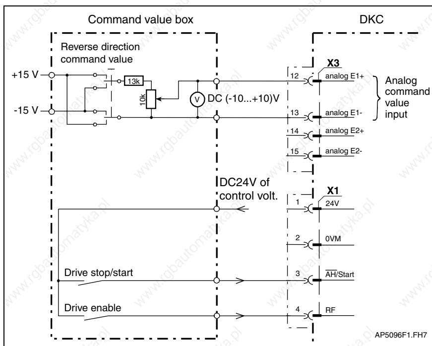
Fig. 16-37: Command value box circuit recommendation for connecting an analog interface
