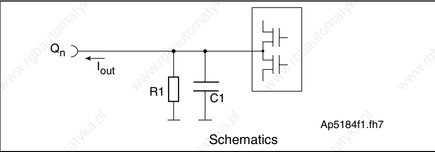
Fig. 4-69: Control outputs
