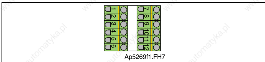
Fig. 4-122: Connector X9
