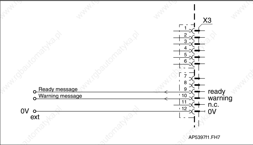
Fig. 5-41: Control outputs
