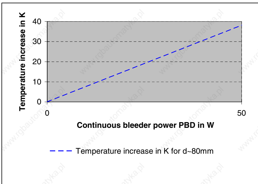
Fig. 12-11: Temperature increase DKC**.3-016-7-FW
