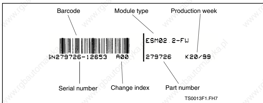
Fig. 14-5: Type plate
