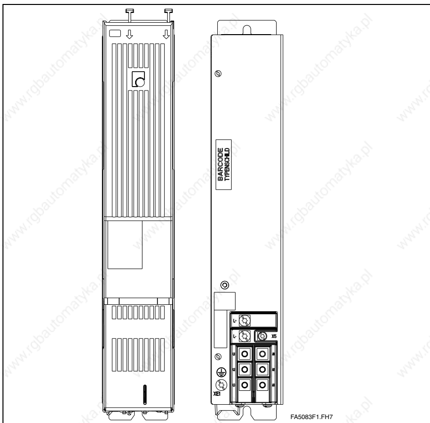
Fig. 7-7: Front view of auxiliary capacitance module CZM01.3
