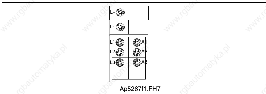
Fig. 6-35: Connector X5
