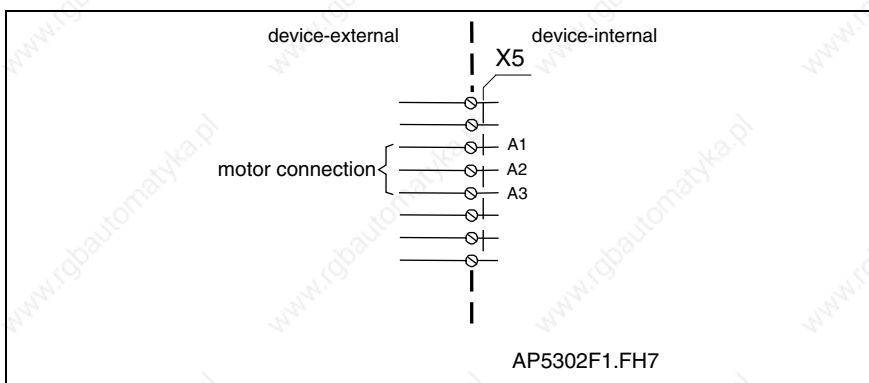
Fig. 4-94: Motor connections
