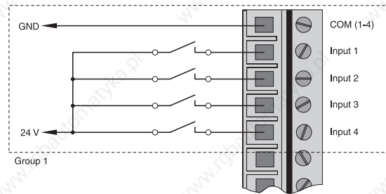
Sink Circuit:
