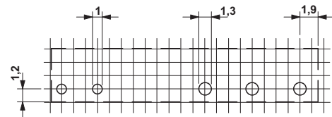
Drilling diagram
