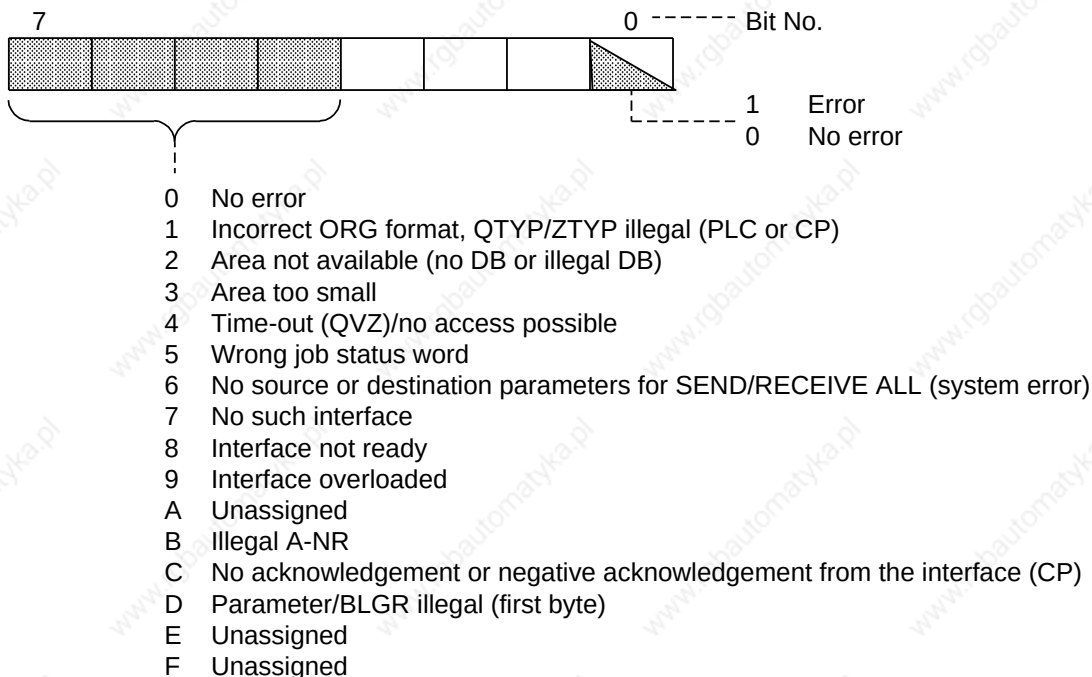
Figure 11-2. Format of the "PAFE" Byte
