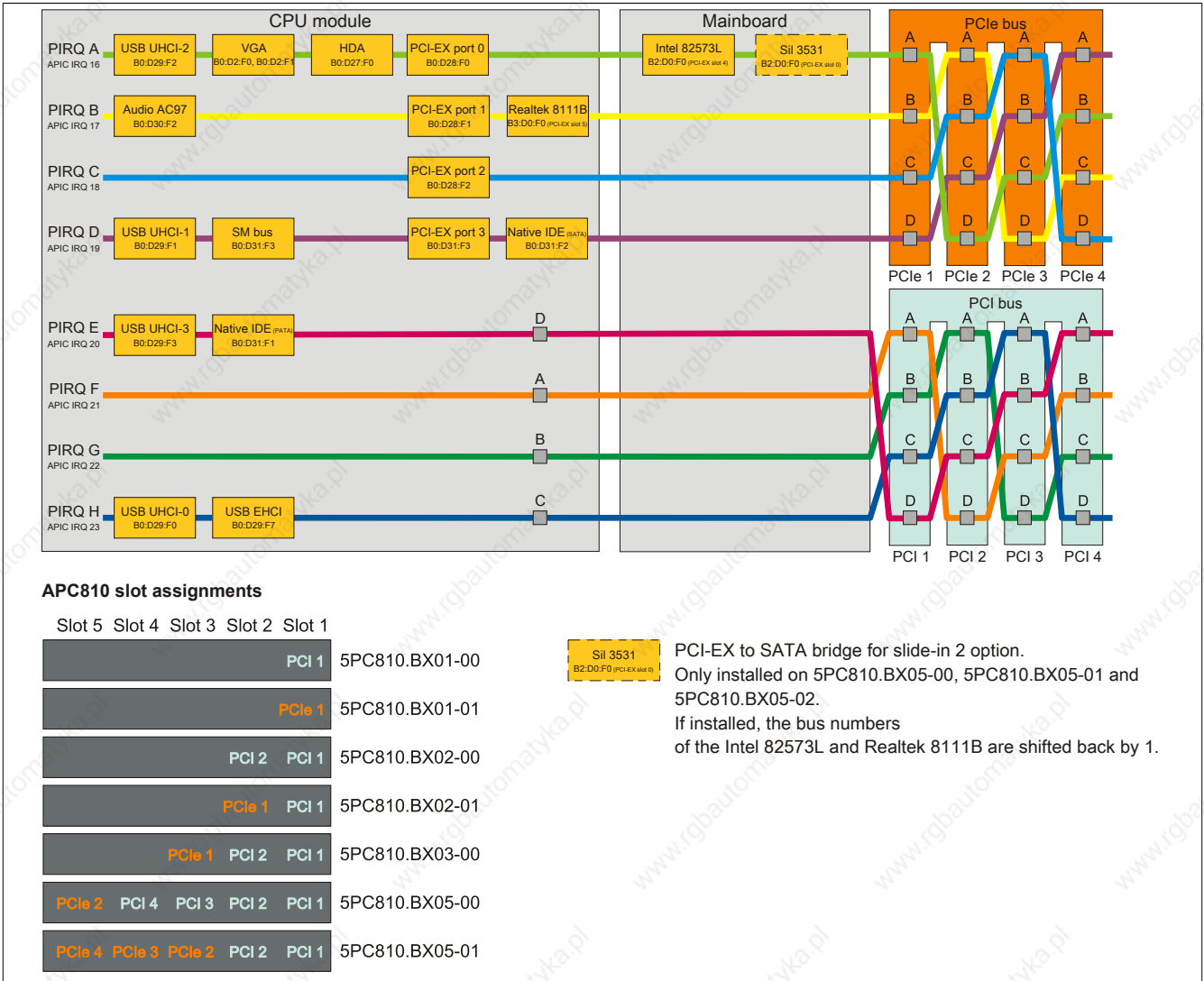
Figure 145: PCI and PCIe routing with enabled 945GME APIC CPU board (COM Express) for BIOS ≥ version 1.14 (bus units 5PC810.BX0x-0x)
