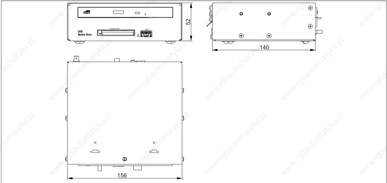
Figure 183: 5MD900.USB2-02 - Dimensions
