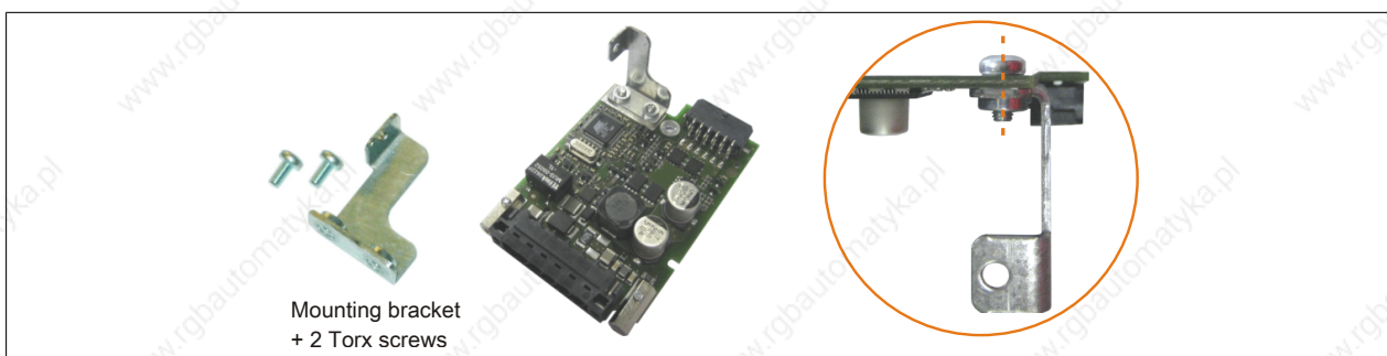
Figure 253: Installing the mounting bracket
