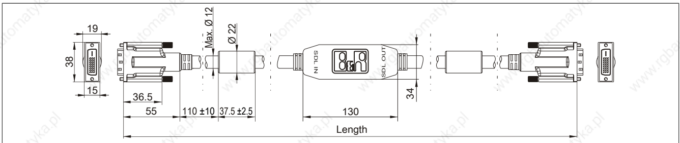
Figure 218: 5CASDL.0xx0-13 - Dimensions
