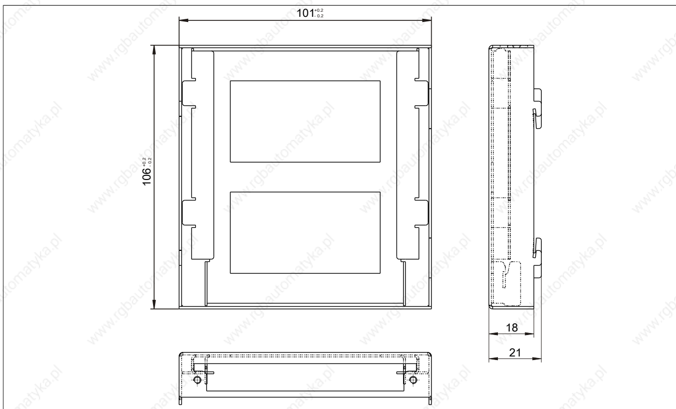
Figure 224: 5AC801.FRAM-00 - Dimensions
