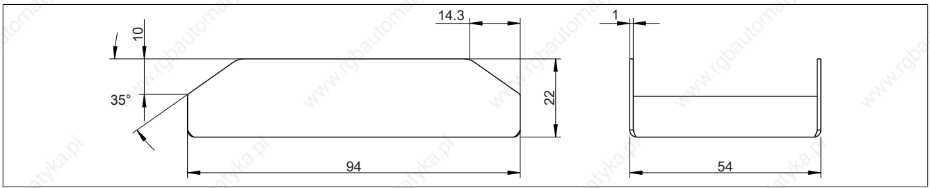
Figure 198: 5AC804.MFLT-00 - Dimensions
