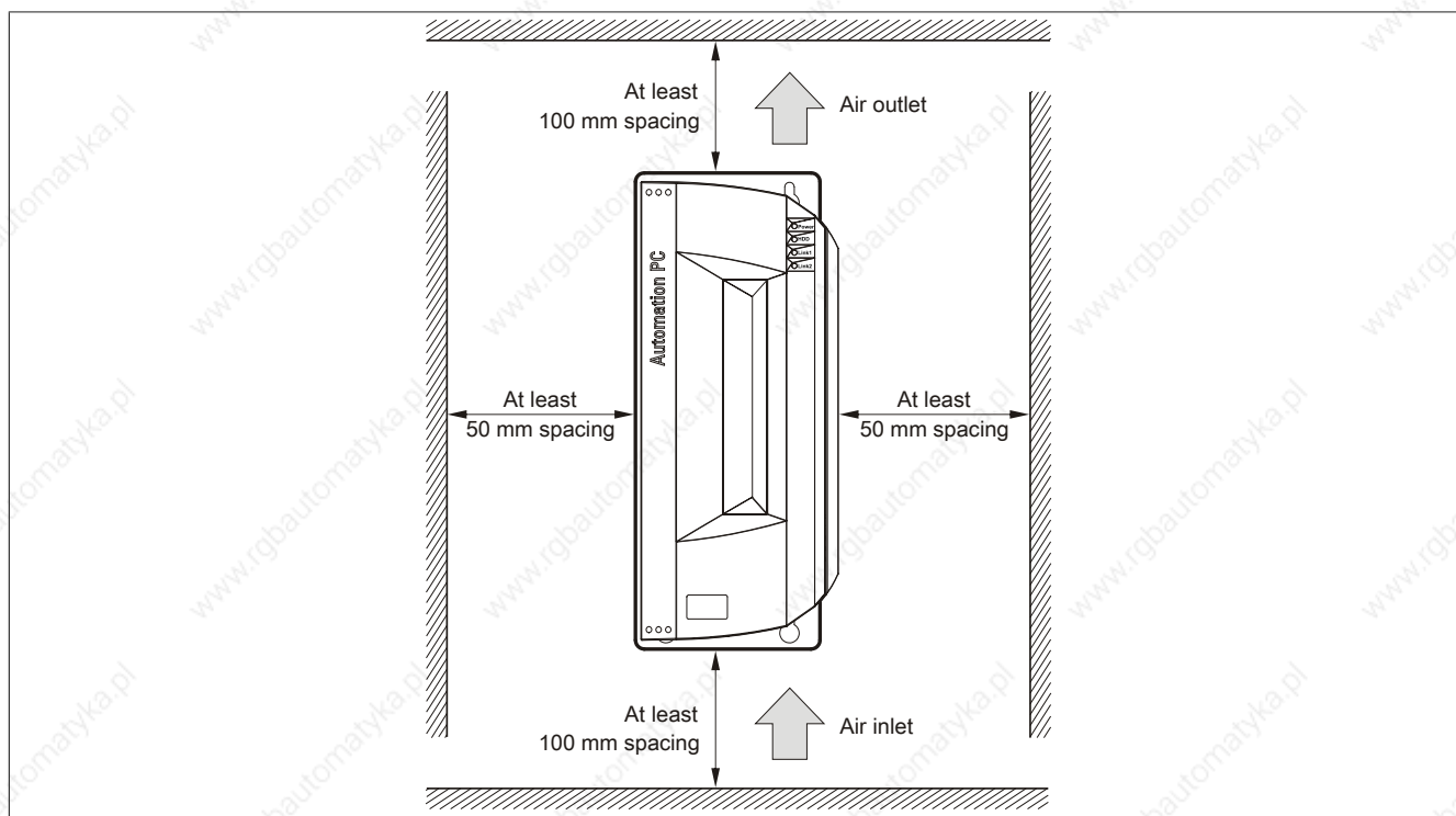
Figure 85: Standard mounting - Spacing
