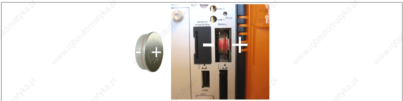
Figure 227: Battery polarity
