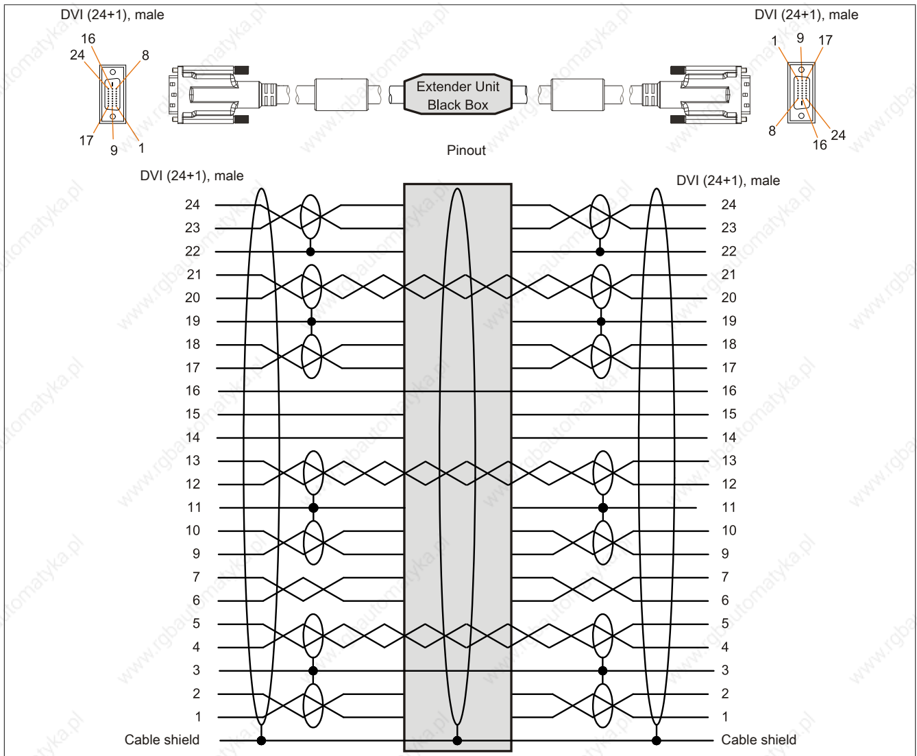
Figure 219: 5CAsDL.0xx0-13 - Pinout
