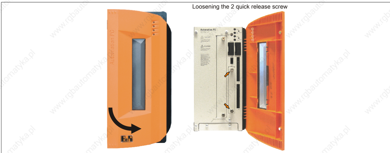
Figure 229: Loosening the quick release screws
