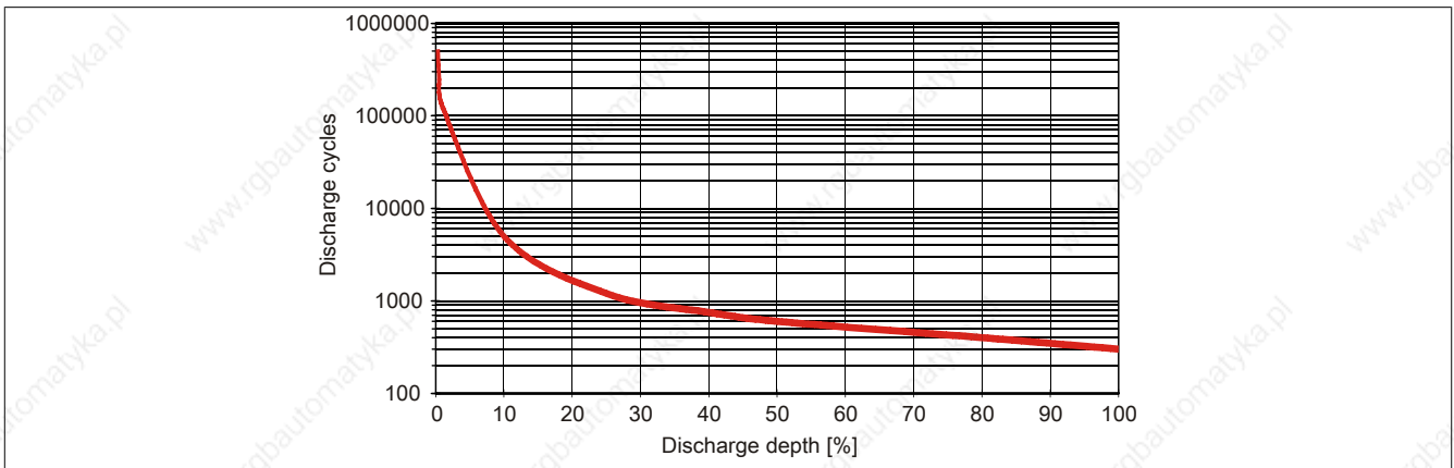
Figure 195: Deep discharge cycles
