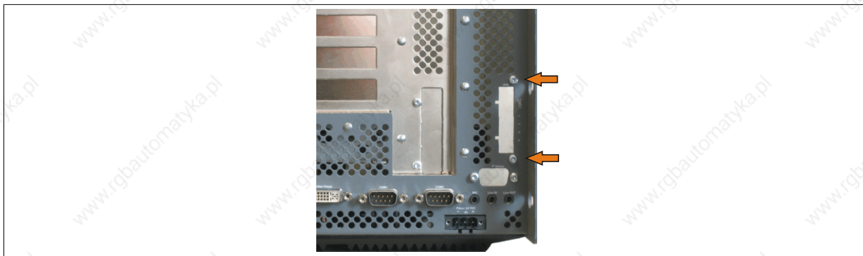
Figure 251: Removing the UPS module cover
