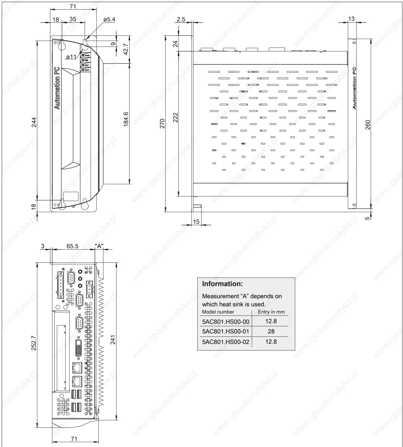
Figure 21: 5PC810.SX01-00 - Dimensions
