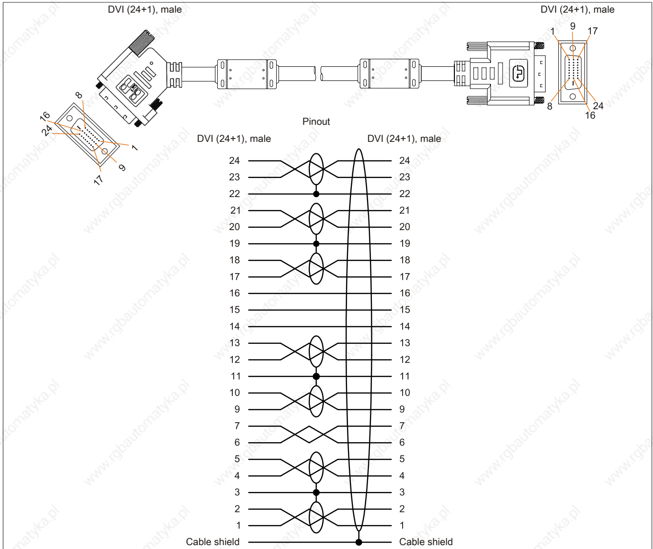
Figure 213: 5CASDL.0xxx-01 - Pinout
