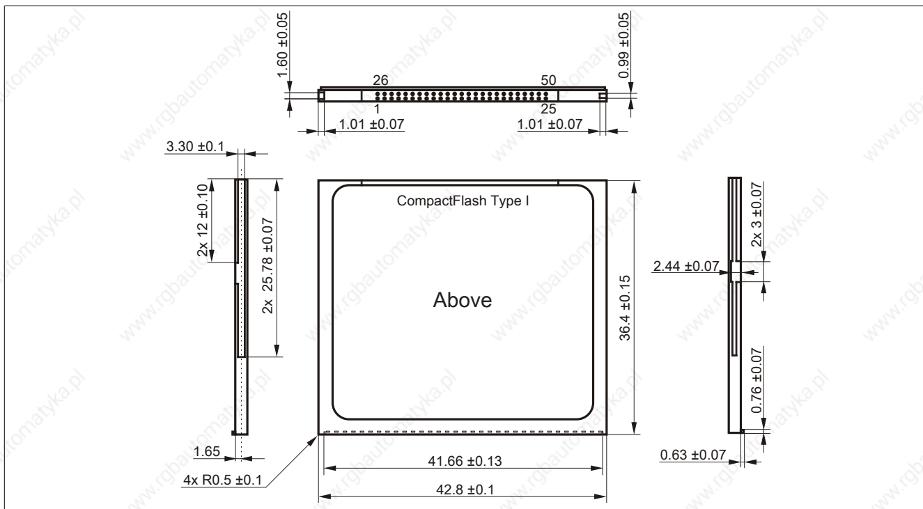
Figure 168: Type I CompactFlash card - Dimensions
