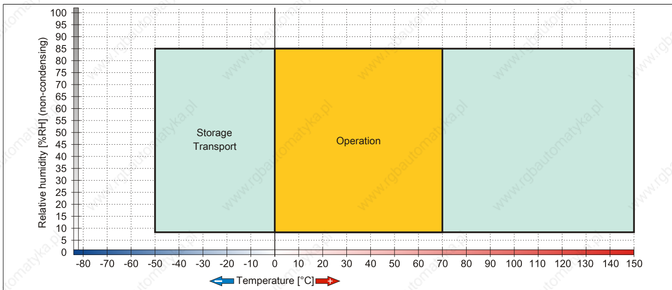
Figure 167: 5CFCRD.xxxx-06 CompactFlash cards - Temperature humidity diagram
