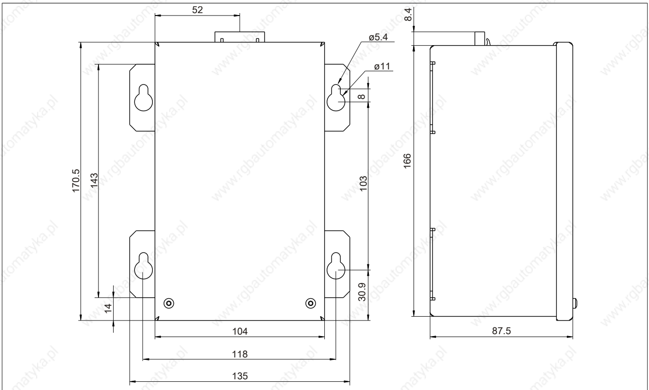
Figure 196: 5PC600.UPSB-00 - Dimensions
