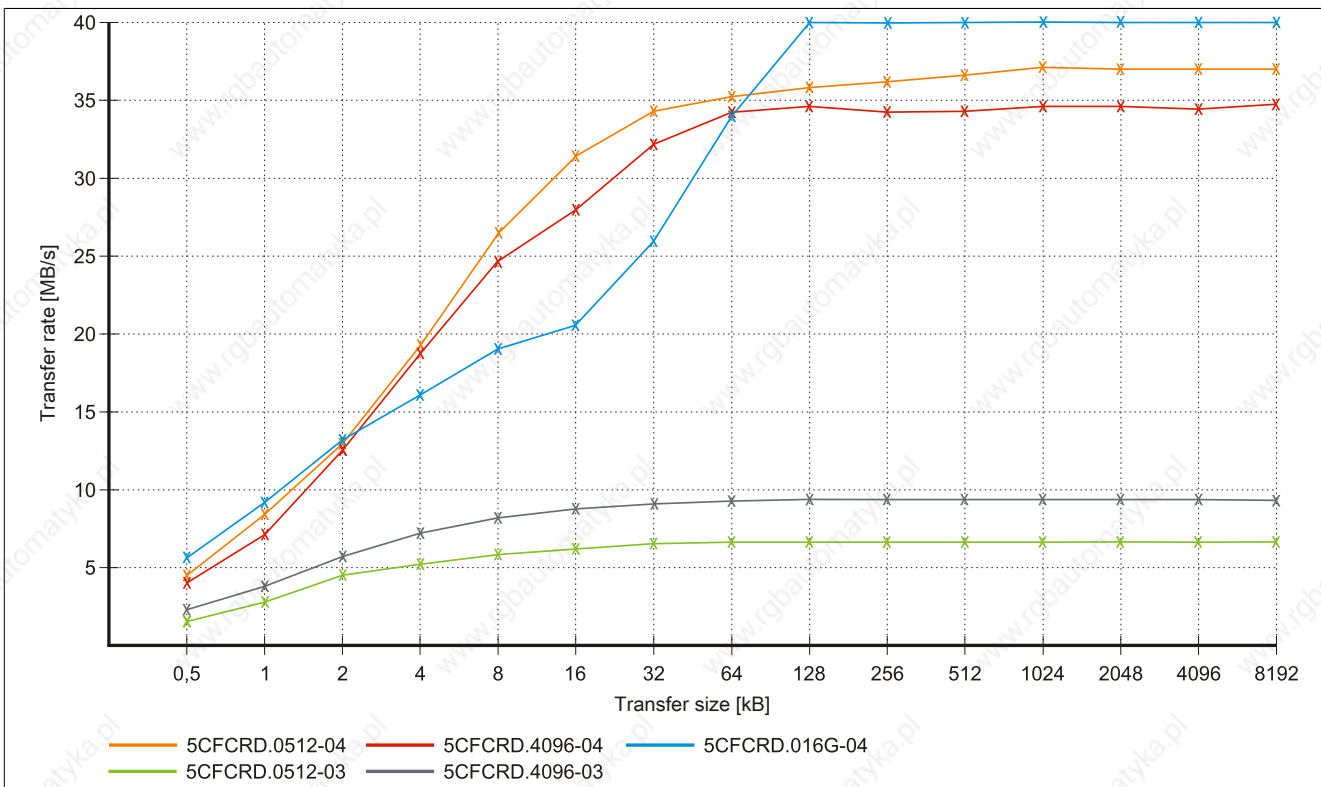
Figure 173: ATTO Disk Benchmark v2.34 read comparison - 5CFCRD.xxxx-03 and 5CFCRD.xxxx-04
