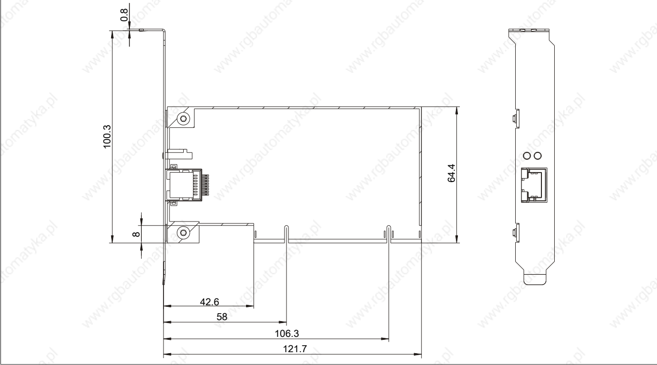
Figure 202: 5ACPCI.ETH1-01 - Dimensions
