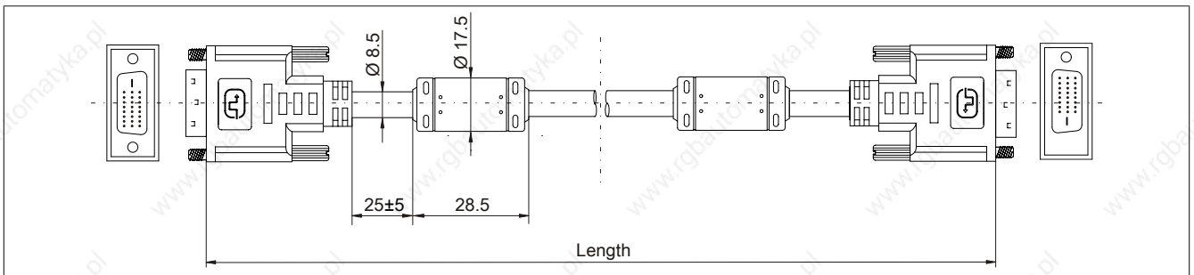
Figure 206: 5CADVI.0xxx-00 - Dimensions
