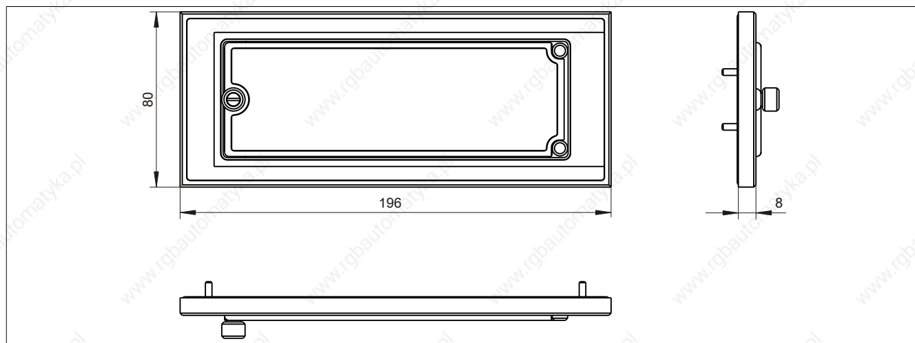
Figure 187: 5A5003.03 - Dimensions
