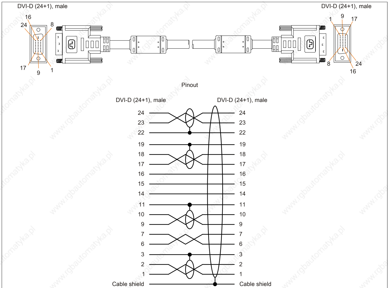
Figure 207: 5CADVI.0xxx-00 - Pinout
