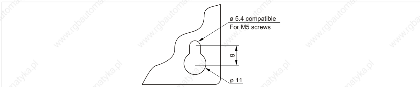
Figure 82: Mounting plates
