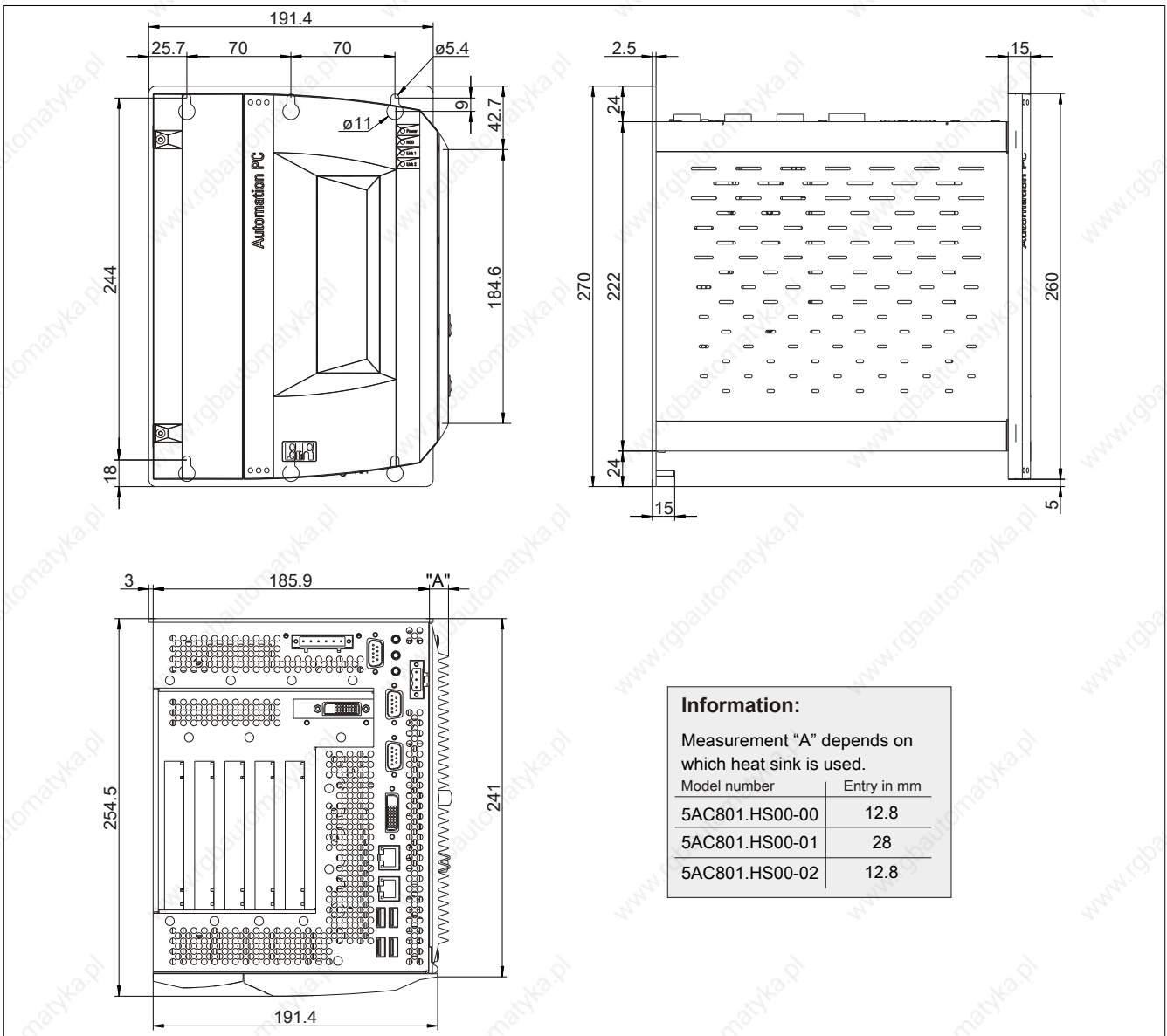
Figure 33: 5PC810.SX05-00 - Dimensions
