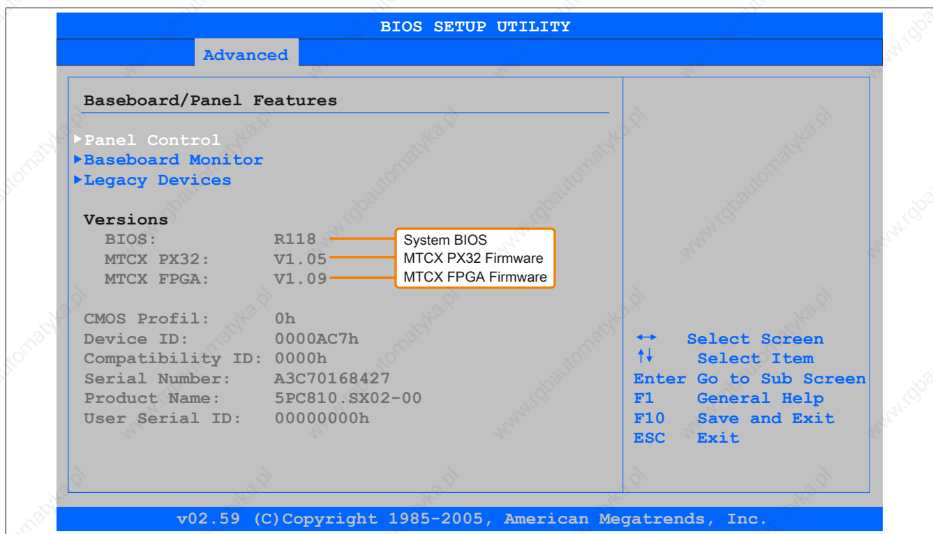
Figure 147: Software version
