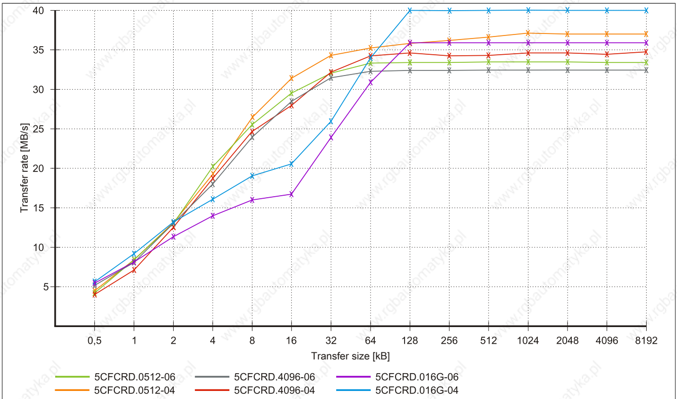
Figure 169: ATTO Disk Benchmark v2.34 read comparison - 5CFCRD.xxxx-04 and 5CFCRD.xxxx-06
