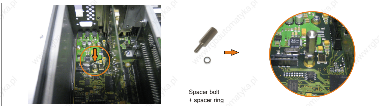
Figure 288: Screwing in the spacing bolt and spacing ring
