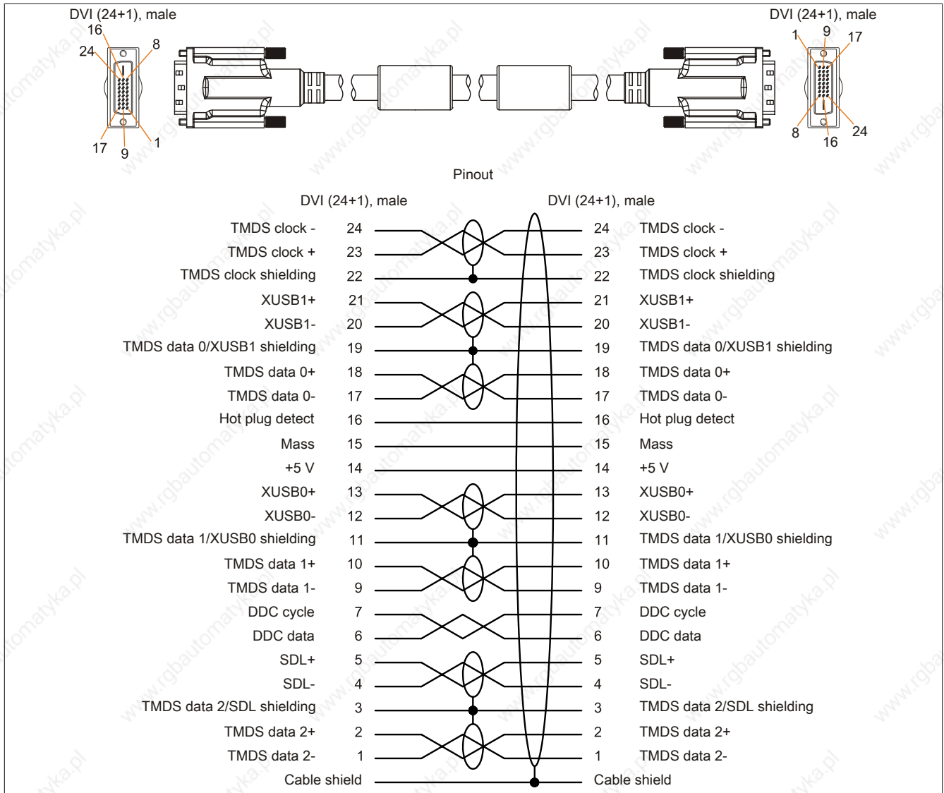
Figure 216: 5CASDL.0xxx-03 - Pinout
