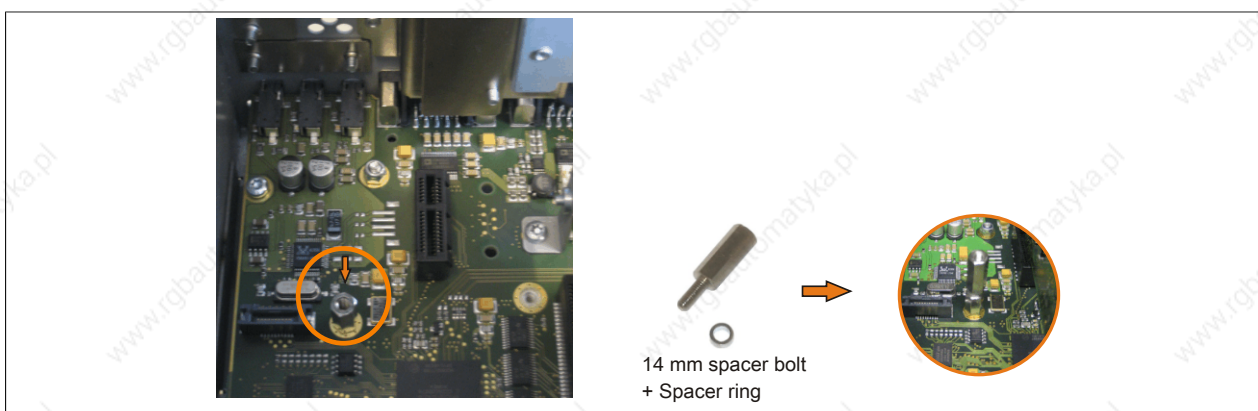
Figure 252: Screwing in the spacing bolt and spacing ring
