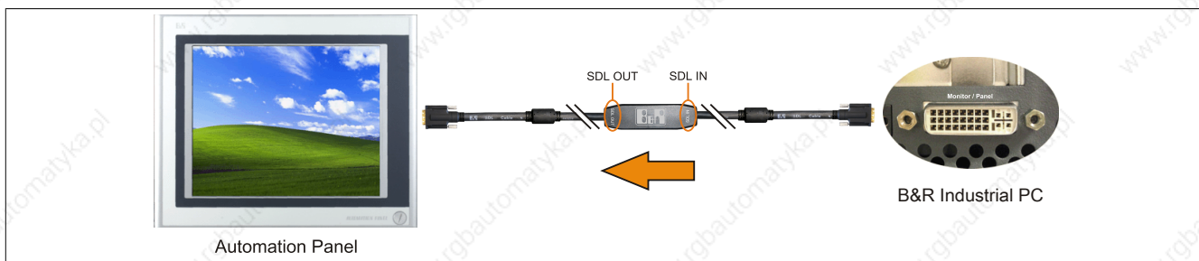
Figure 220: Example of the signal direction for an SDL flex cable with extender
