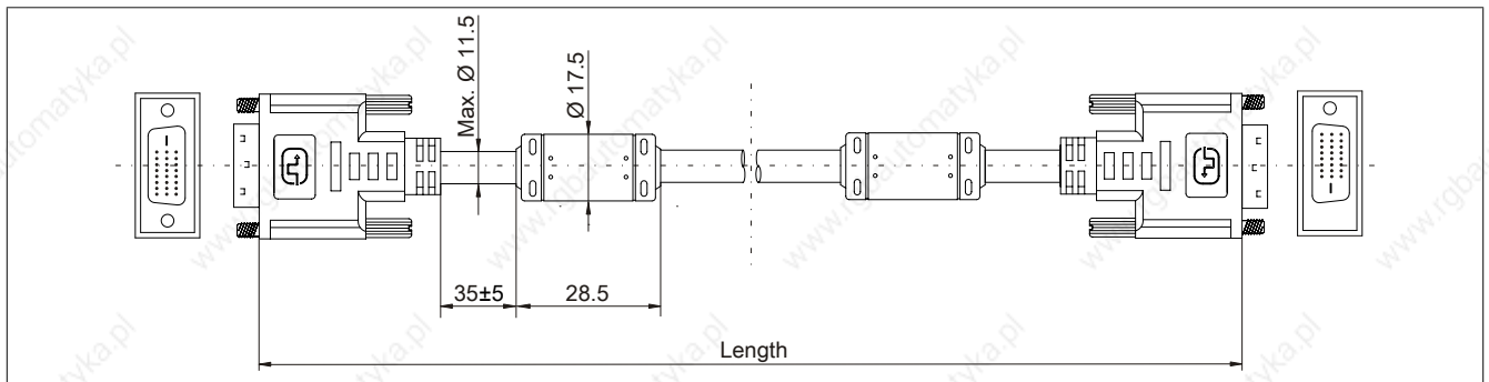
Figure 209: 5CASDL.0xxx-00- Dimensions
