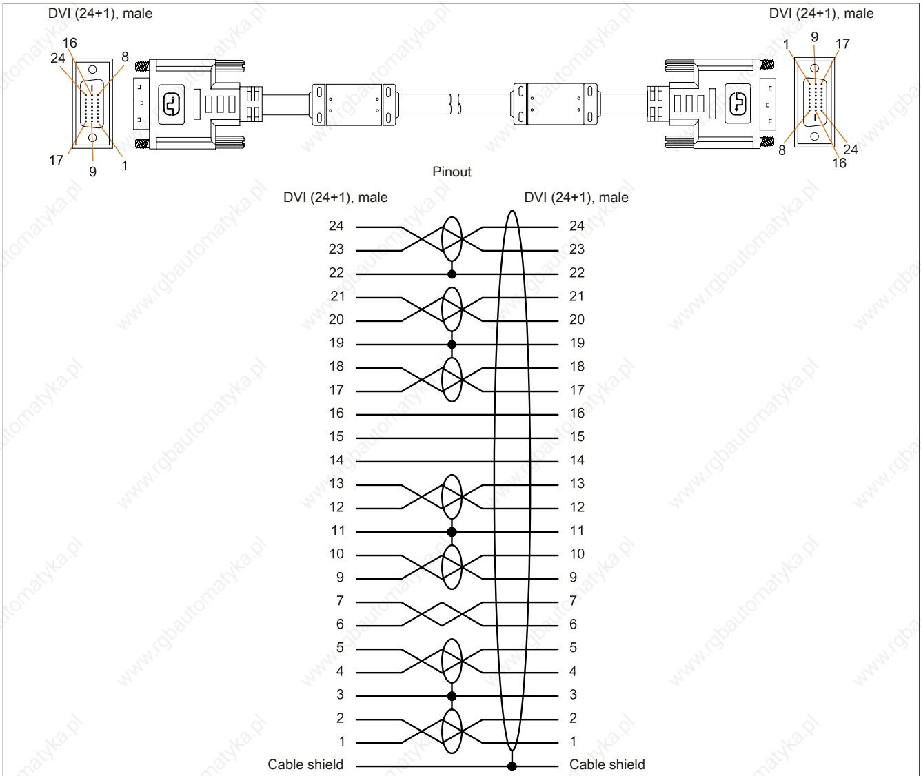
Figure 210: 5CASDL.0xxx-00 - Pinout
