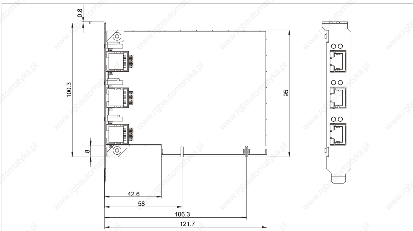
Figure 204: 5ACPCI.ETH3-01 - Dimensions
