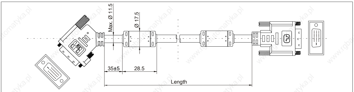
Figure 212: 5CASDL.0xxx-01 - Dimensions
