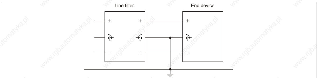
Figure 200: Connection example
