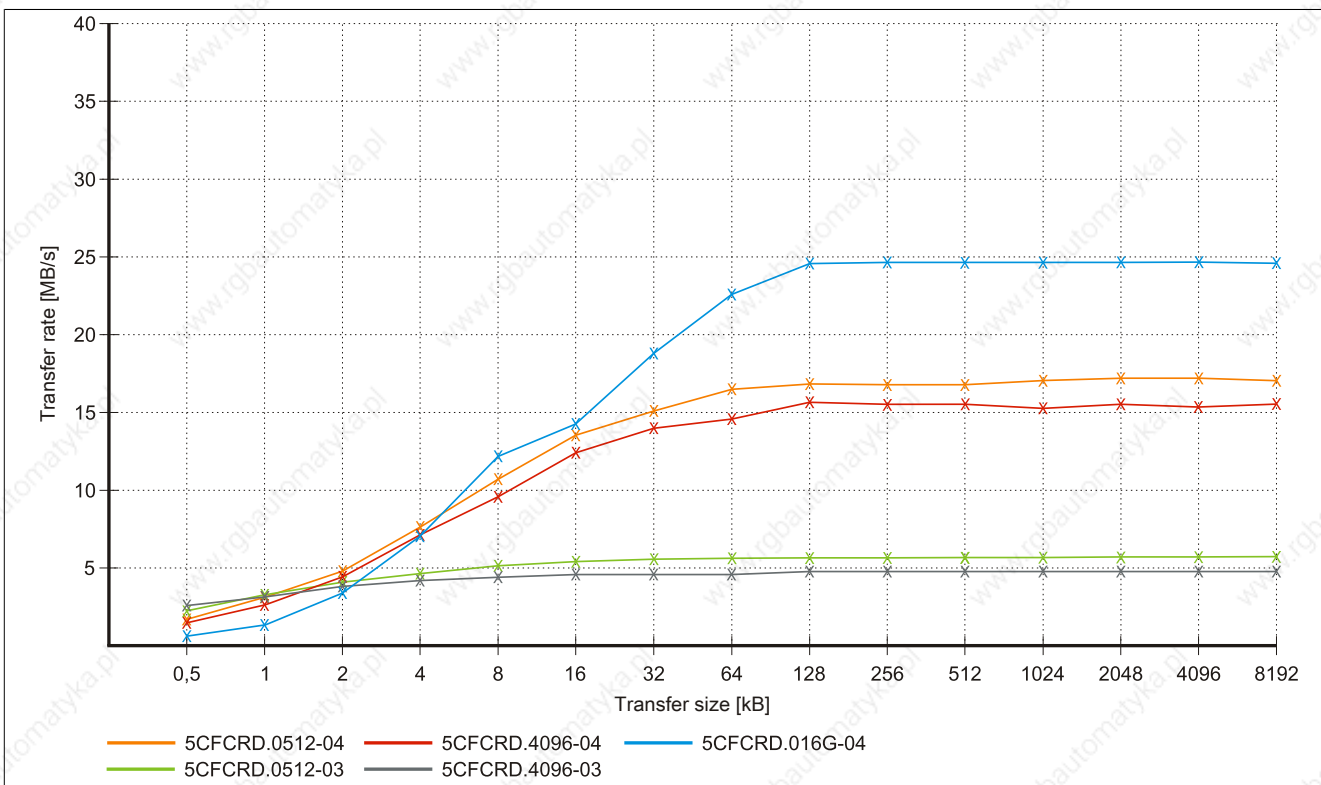
Figure 174: ATTO Disk Benchmark v2.34 write comparison - 5CFCRD.xxxx-03 and 5CFCRD.xxxx-04
