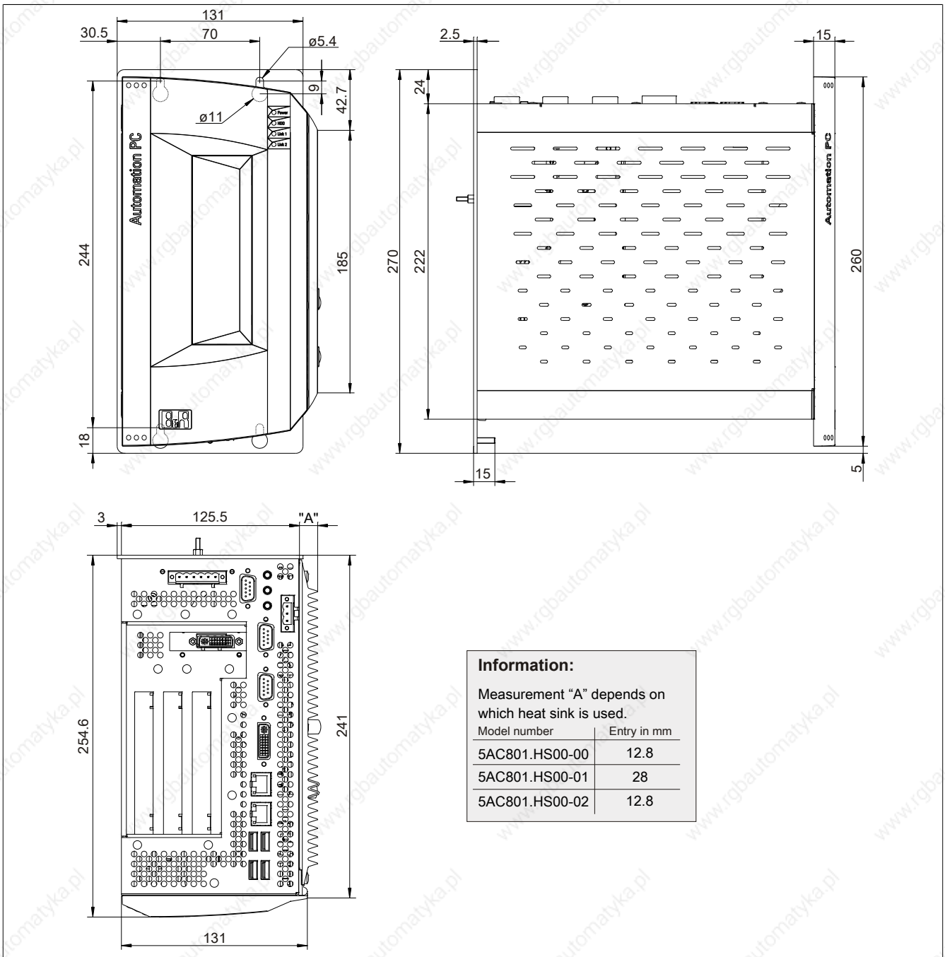
Figure 29: 5PC810.SX03-00 - Dimensions
