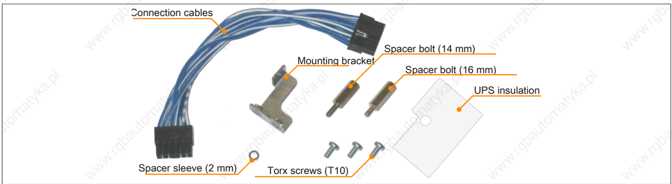
Figure 239: 5AC600. UPSI-00 Add-on UPS module - Installation materials
