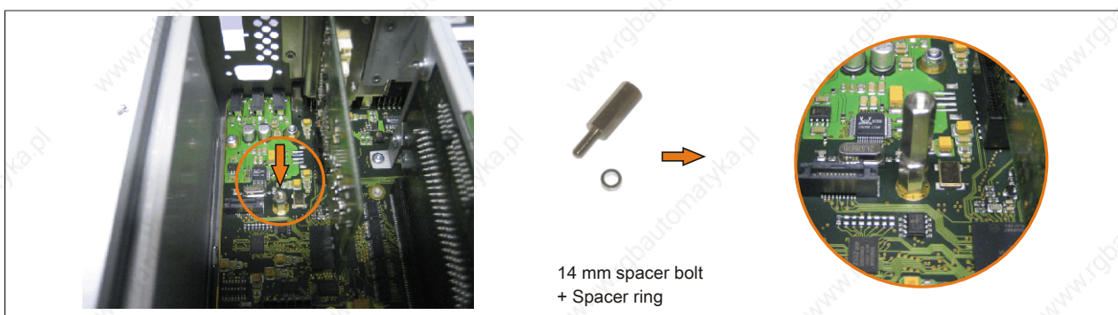
Figure 246: Screwing in the spacing bolt and spacing ring
