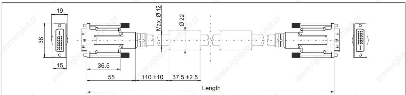
Figure 215: 5CASDL.0xxx-03 - Dimensions
