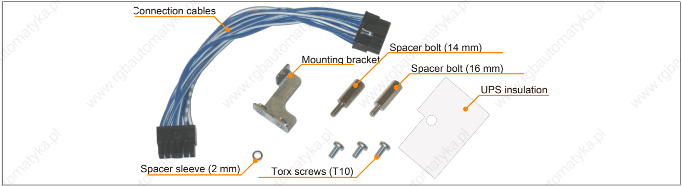
Figure 193: 5AC600. UPSI-00 Add-on UPS module - Installation materials
