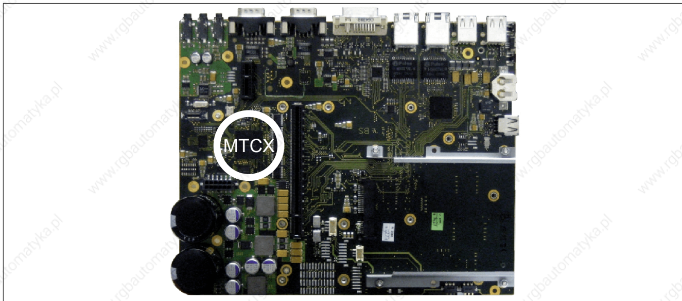
Figure 291: MTCX controller location
