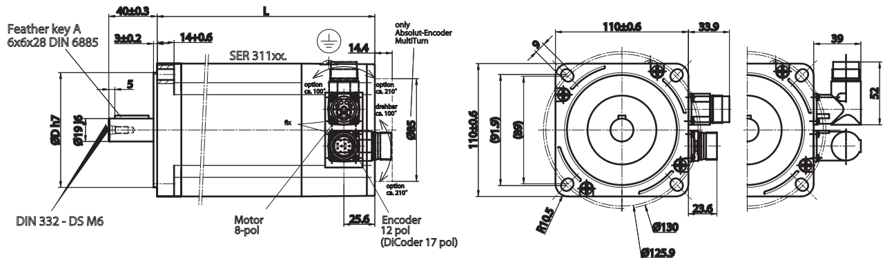
Dimensions SER311x
