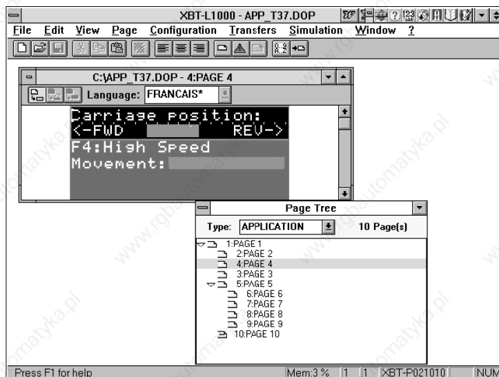
Figure 42: Application Page 3
