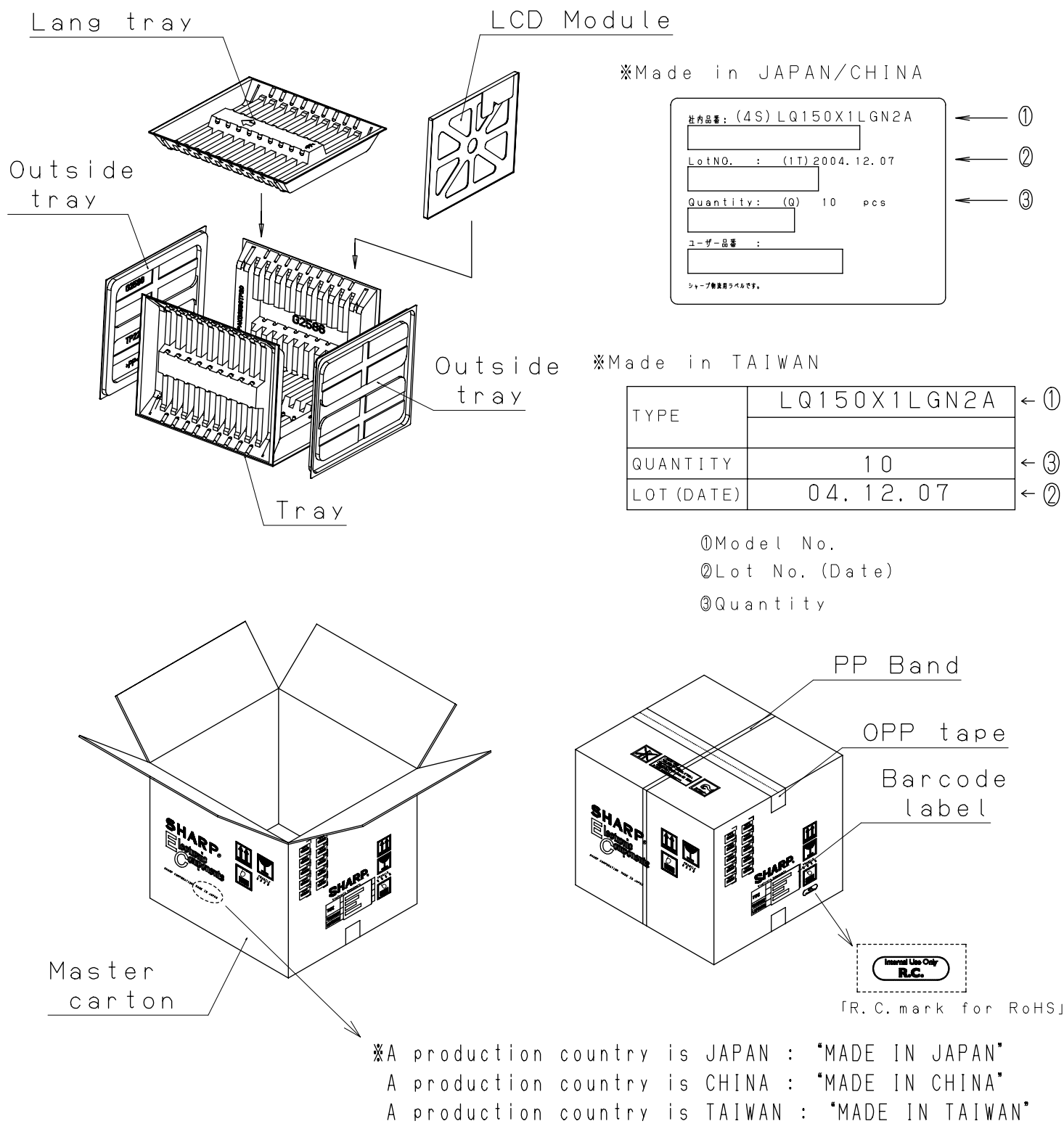
Fig.3 Packing Form (LQ150X1LGN2A)
