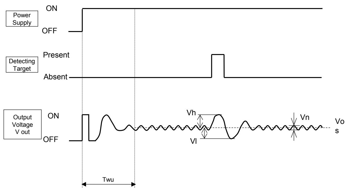
4-4 Timing Chart
