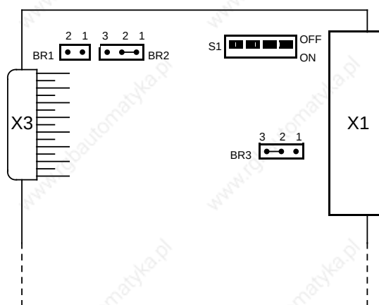
Figure 3-23. Jumper Settings on the IM 314
