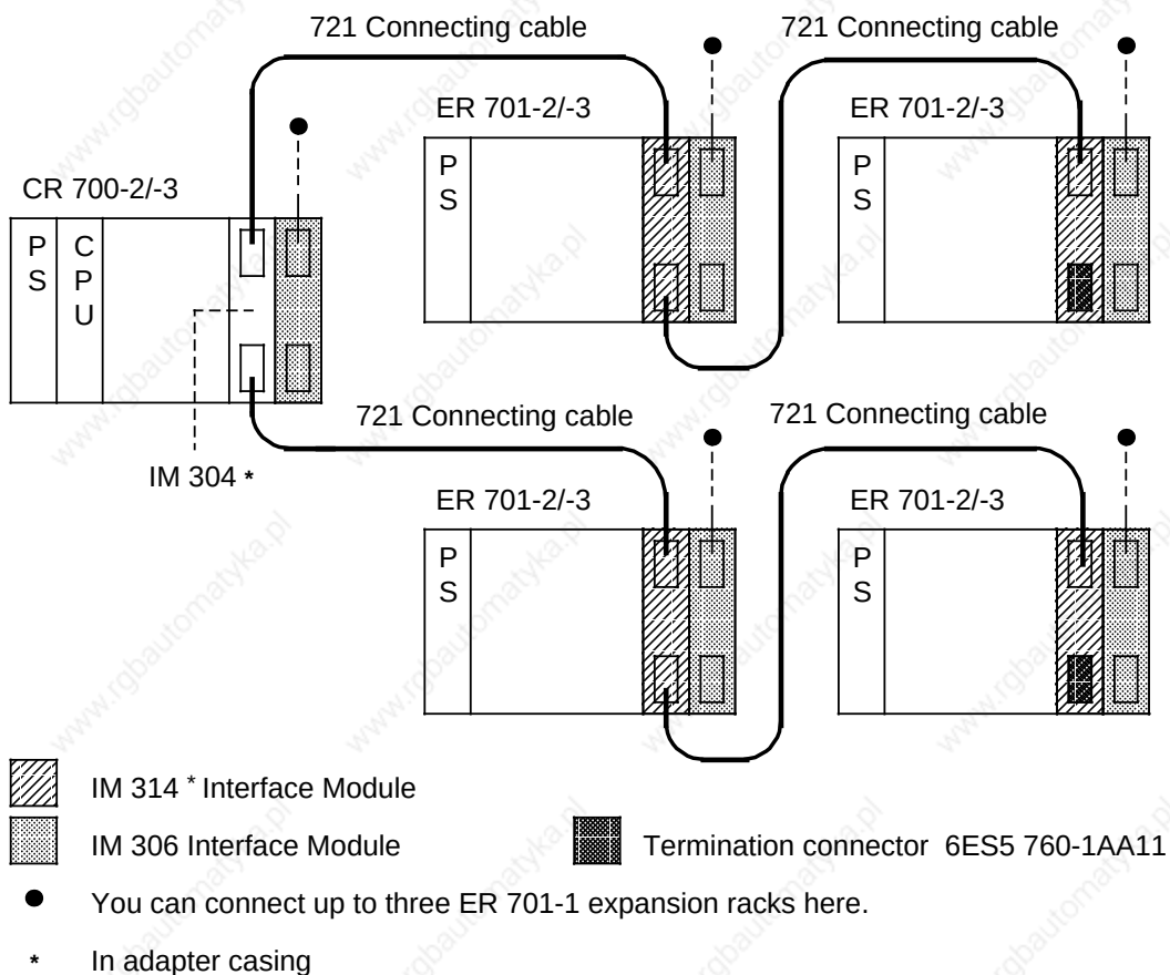
Figure 3- 20. Distributed Configuration with IM 304/IM 314
