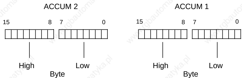
Figure 8-1. Accumulator Structure
