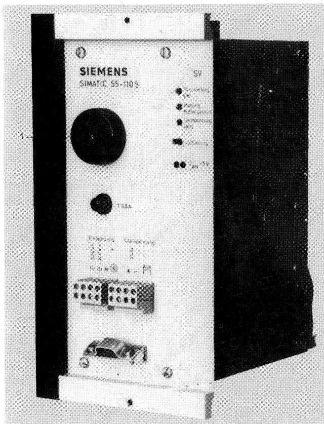
Fig. 12 Power supply unit
