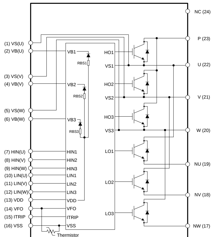
Internal Electrical Schematic
