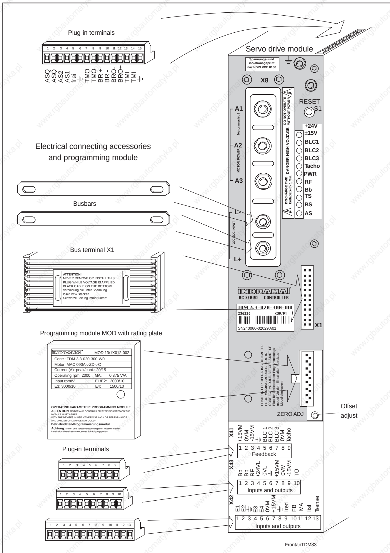
Figure 7: Front view of TDM 3.3
