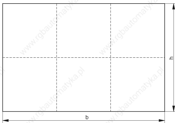
Diagram 5: PANELWARE cutout size example
