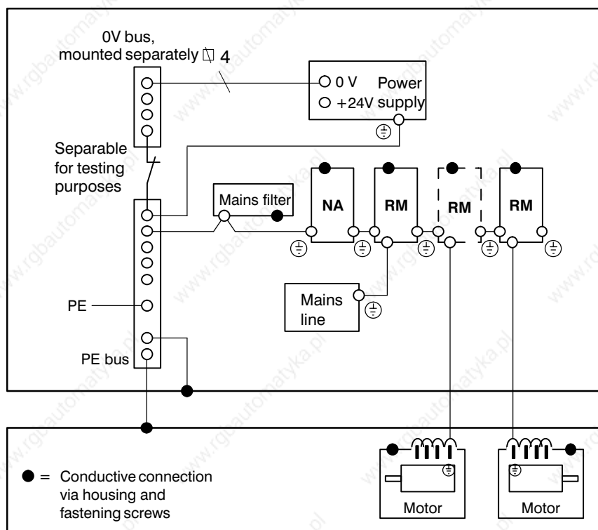
Fig. 2.6: Earthing plan Servodyn-D with VM...B,C,D
