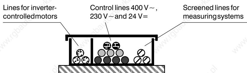
Fig. 4.1: Cable duct with two chambers
