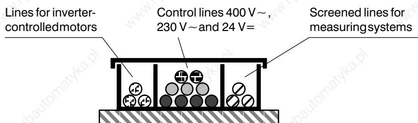
Fig. 4.2: Cable duct with three chambers, necessary for employment of sensitive measuring systems with sinusoidal signal transmission
