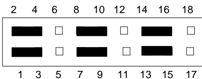
Configuration #8: 1M x 8 ROM/PROM/EPROM
