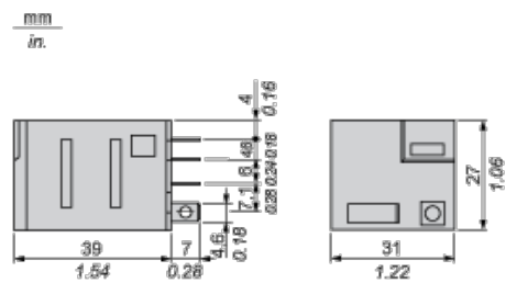
Pin Side View
